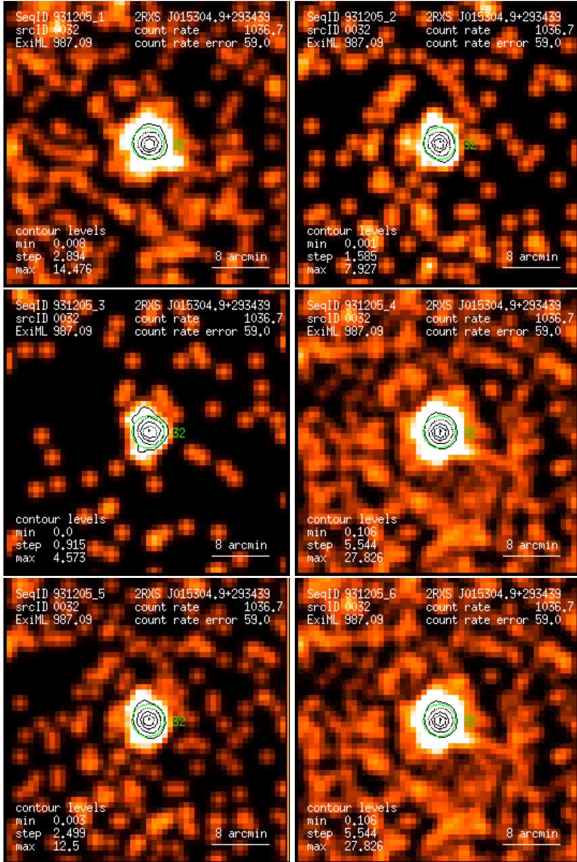
Figure 32: RASS 931205: detection 0032: band rate images, Gaussian filter: (1) PSPC channels 11 – 41, (2) 52 – 90, (3) 91 – 201, (4) 11 – 235, (5) 52 – 201, (6) 11 – 201. Broad band rates in counts/ks. Band rate contour levels in counts/ks/arcmin 2 .
