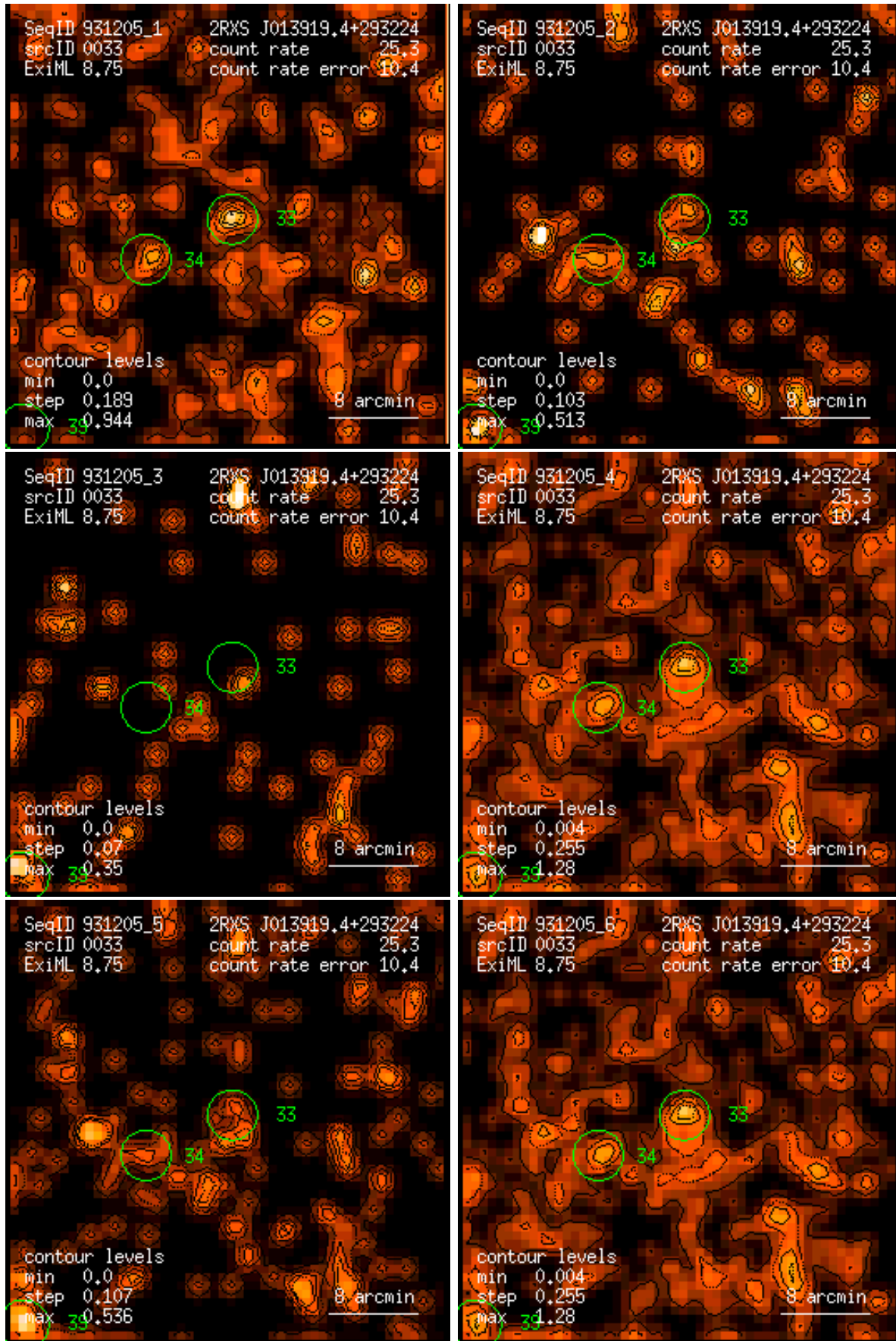
Figure 33: RASS 931205: detection 0033: band rate images, Gaussian filter: (1) PSPC channels 11 – 41, (2) 52 – 90, (3) 91 – 201, (4) 11 – 235, (5) 52 – 201, (6) 11 – 201. Broad band rates in counts/ks. Band rate contour levels in counts/ks/arcmin 2 .
