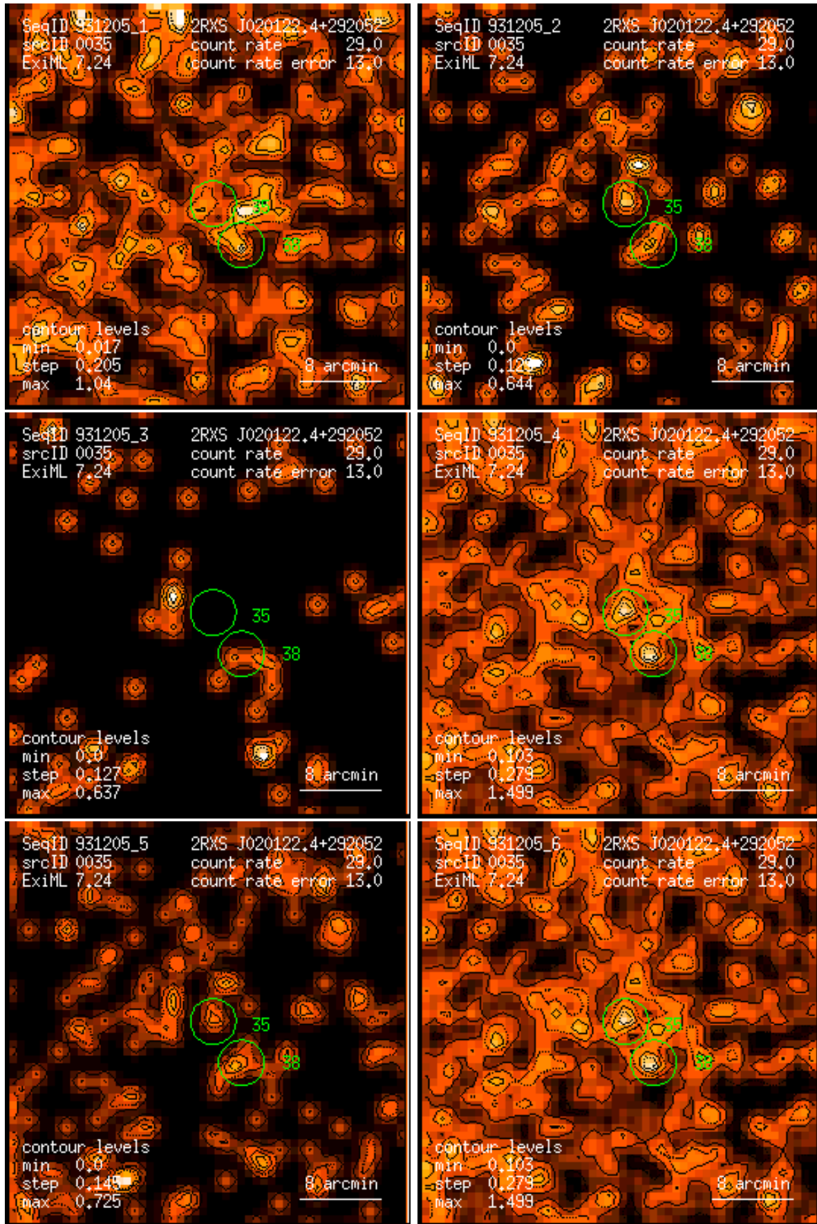
Figure 35: RASS 931205: detection 0035: band rate images, Gaussian filter: (1) PSPC channels 11 – 41, (2) 52 – 90, (3) 91 – 201, (4) 11 – 235, (5) 52 – 201, (6) 11 – 201. Broad band rates in counts/ks. Band rate contour levels in counts/ks/arcmin 2 .
