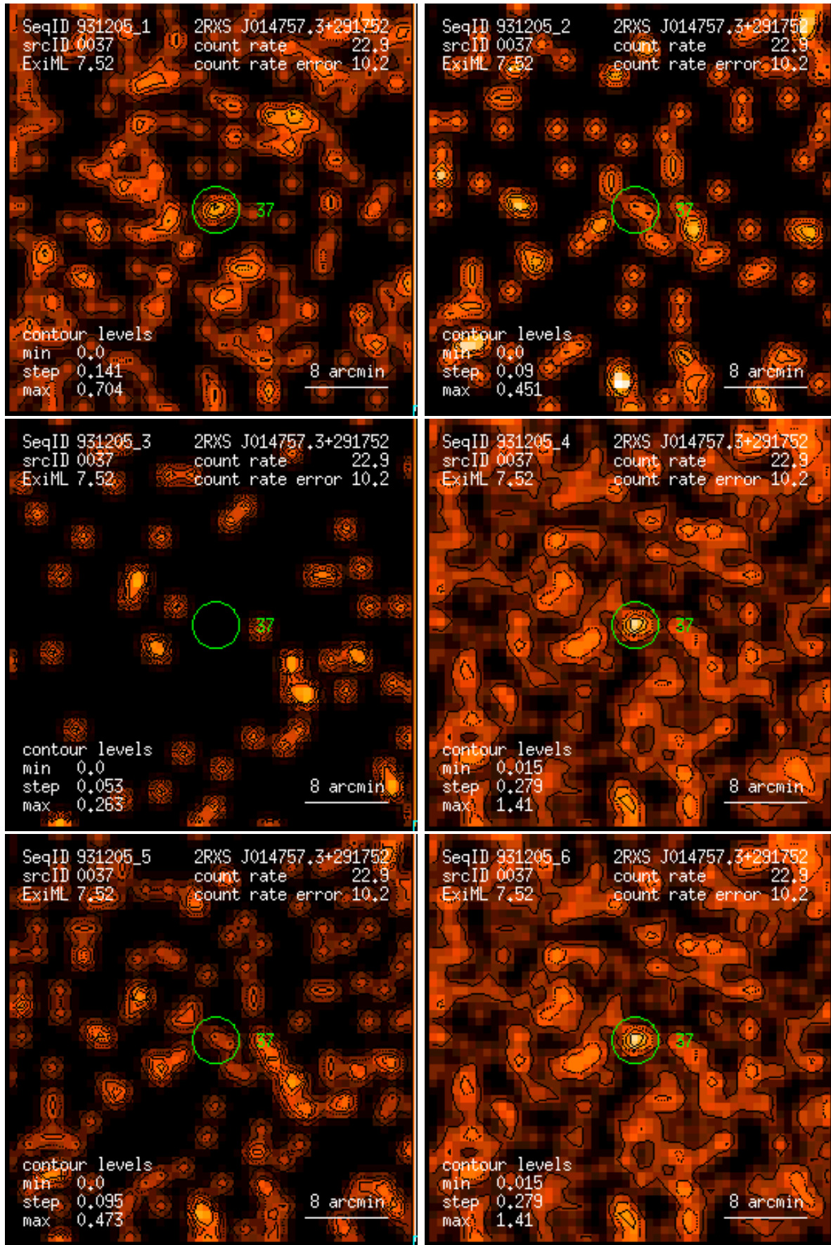
Figure 37: RASS 931205: detection 0037: band rate images, Gaussian filter: (1) PSPC channels 11 – 41, (2) 52 – 90, (3) 91 – 201, (4) 11 – 235, (5) 52 – 201, (6) 11 – 201. Broad band rates in counts/ks. Band rate contour levels in counts/ks/arcmin 2 .
