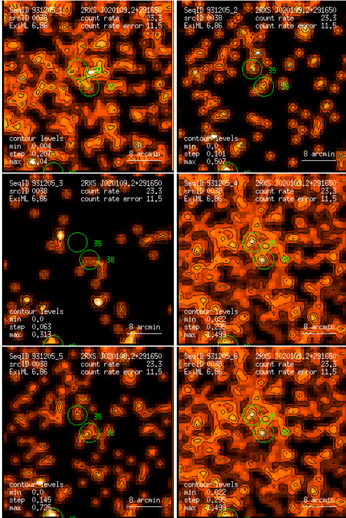
Figure 38: RASS 931205: detection 0038: band rate images, Gaussian filter: (1) PSPC channels 11 – 41, (2) 52 – 90, (3) 91 – 201, (4) 11 – 235, (5) 52 – 201, (6) 11 – 201. Broad band rates in counts/ks. Band rate contour levels in counts/ks/arcmin 2 .
