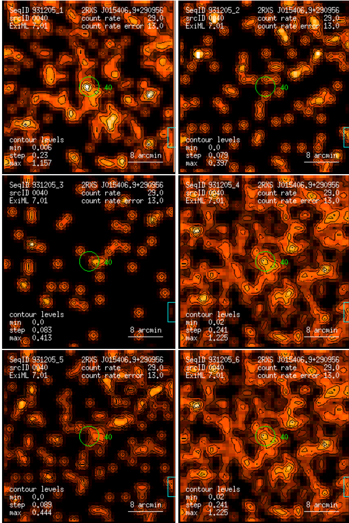
Figure 40: RASS 931205: detection 0040: band rate images, Gaussian filter: (1) PSPC channels 11 – 41, (2) 52 – 90, (3) 91 – 201, (4) 11 – 235, (5) 52 – 201, (6) 11 – 201. Broad band rates in counts/ks. Band rate contour levels in counts/ks/arcmin 2 .
