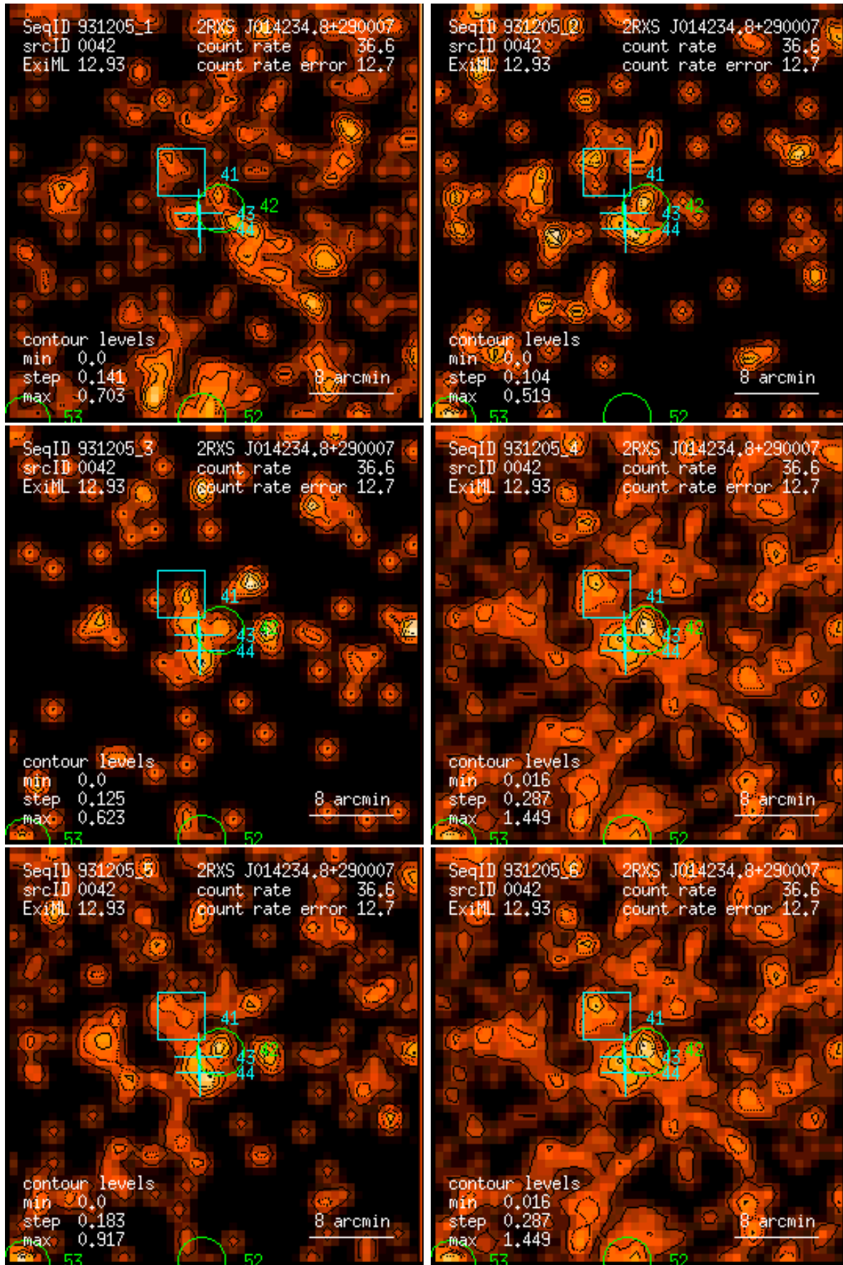
Figure 42: RASS 931205: detection 0042: band rate images, Gaussian filter: (1) PSPC channels 11 – 41, (2) 52 – 90, (3) 91 – 201, (4) 11 – 235, (5) 52 – 201, (6) 11 – 201. Broad band rates in counts/ks. Band rate contour levels in counts/ks/arcmin 2 .
