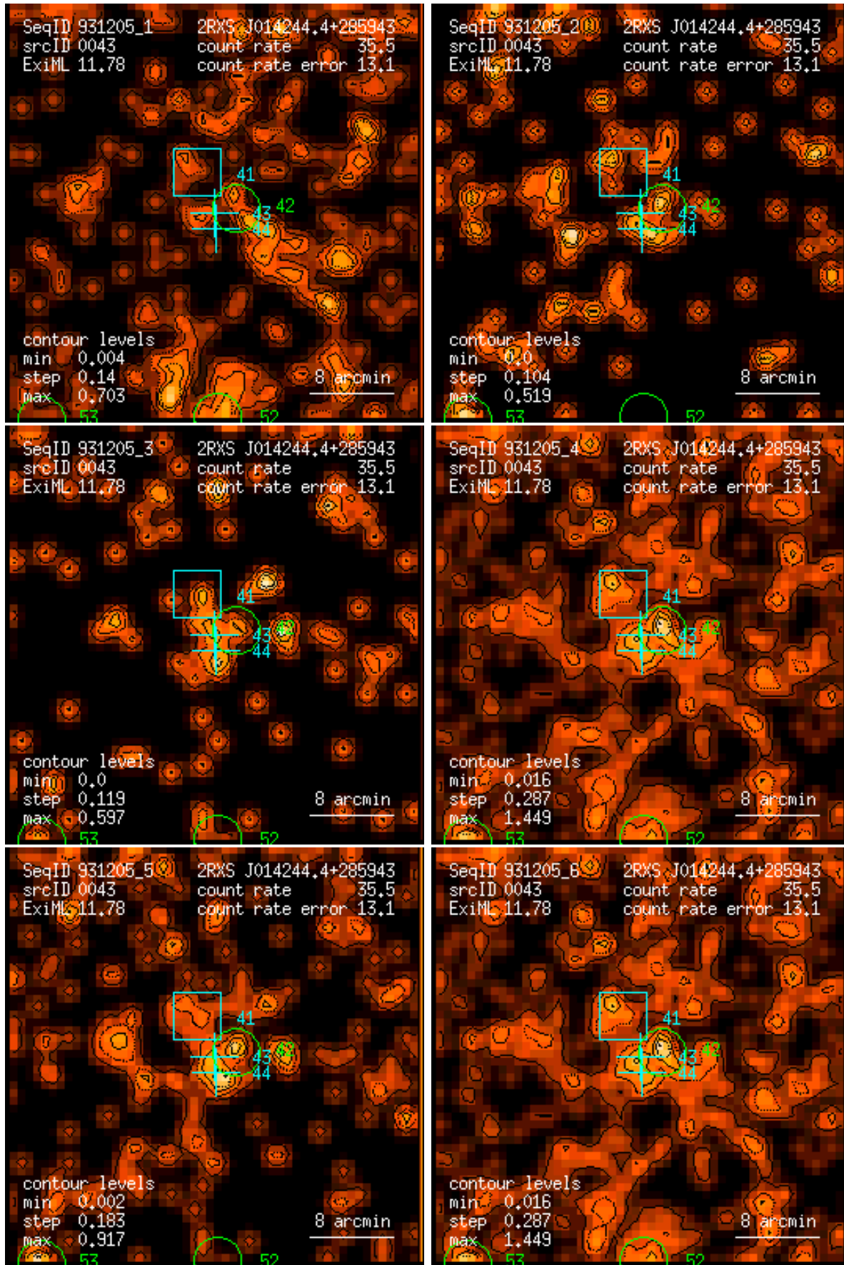
Figure 43: RASS 931205: detection 0043: band rate images, Gaussian filter: (1) PSPC channels 11 – 41, (2) 52 – 90, (3) 91 – 201, (4) 11 – 235, (5) 52 – 201, (6) 11 – 201. Broad band rates in counts/ks. Band rate contour levels in counts/ks/arcmin 2 .
