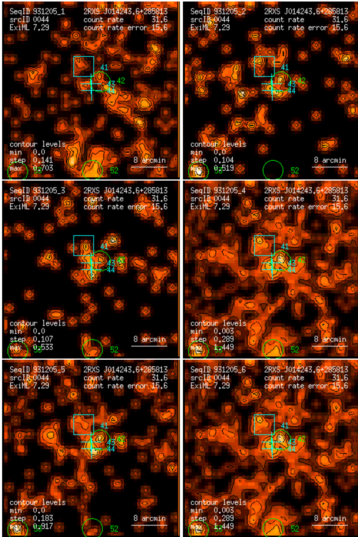
Figure 44: RASS 931205: detection 0044: band rate images, Gaussian filter: (1) PSPC channels 11 – 41, (2) 52 – 90, (3) 91 – 201, (4) 11 – 235, (5) 52 – 201, (6) 11 – 201. Broad band rates in counts/ks. Band rate contour levels in counts/ks/arcmin 2 .
