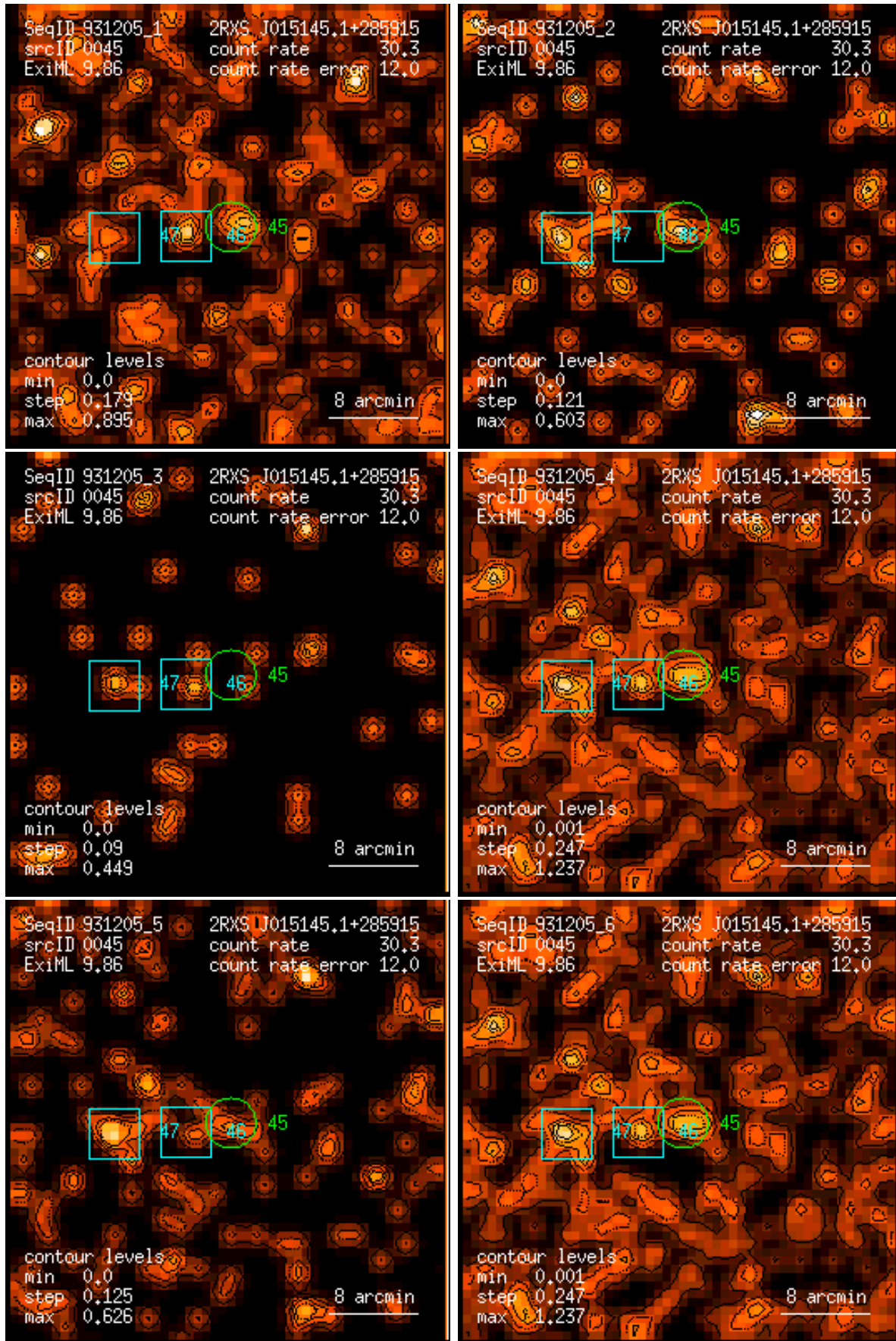
Figure 45: RASS 931205: detection 0045: band rate images, Gaussian filter: (1) PSPC channels 11 – 41, (2) 52 – 90, (3) 91 – 201, (4) 11 – 235, (5) 52 – 201, (6) 11 – 201. Broad band rates in counts/ks. Band rate contour levels in counts/ks/arcmin 2 .
