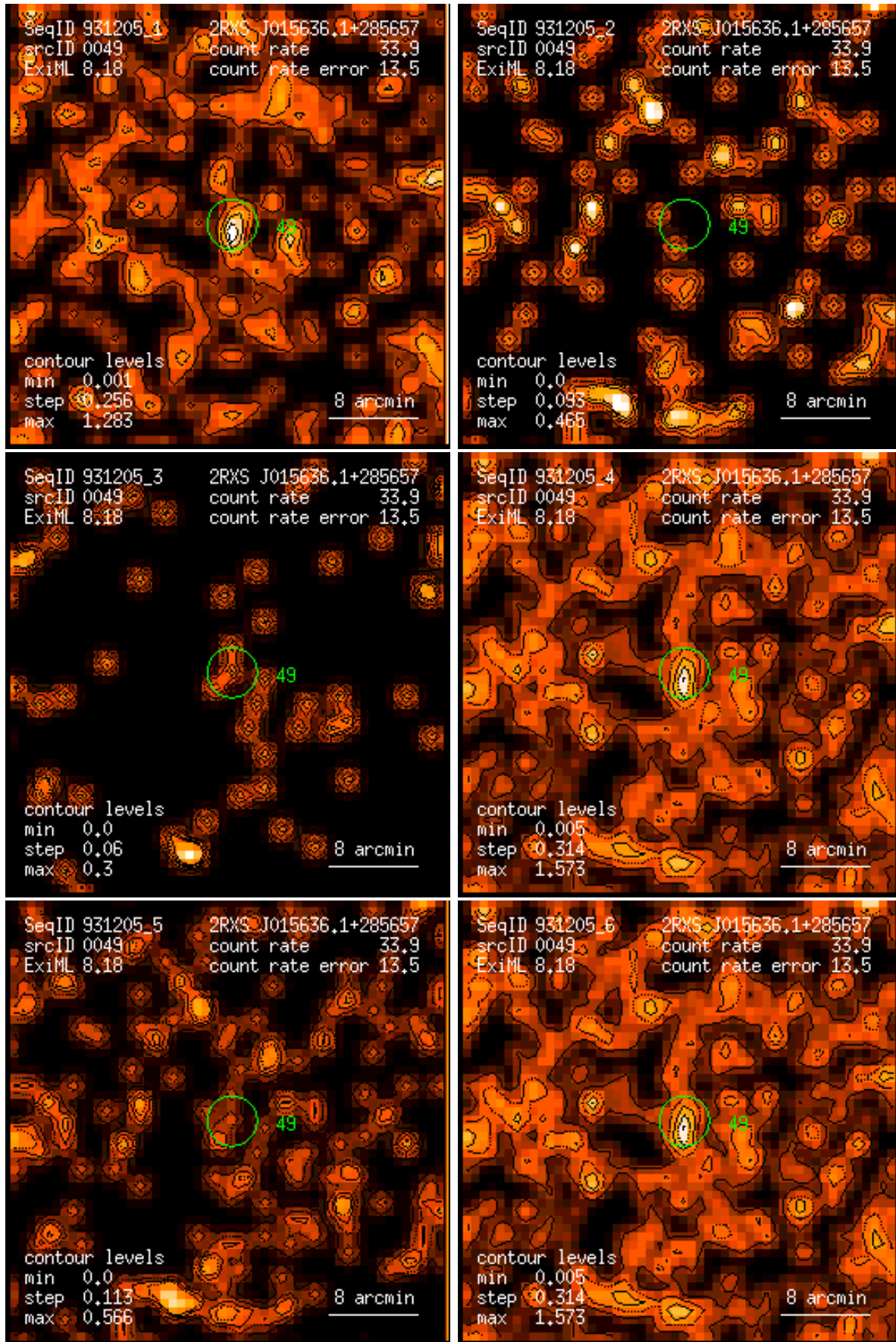
Figure 49: RASS 931205: detection 0049: band rate images, Gaussian filter: (1) PSPC channels 11 – 41, (2) 52 – 90, (3) 91 – 201, (4) 11 – 235, (5) 52 – 201, (6) 11 – 201. Broad band rates in counts/ks. Band rate contour levels in counts/ks/arcmin 2 .
