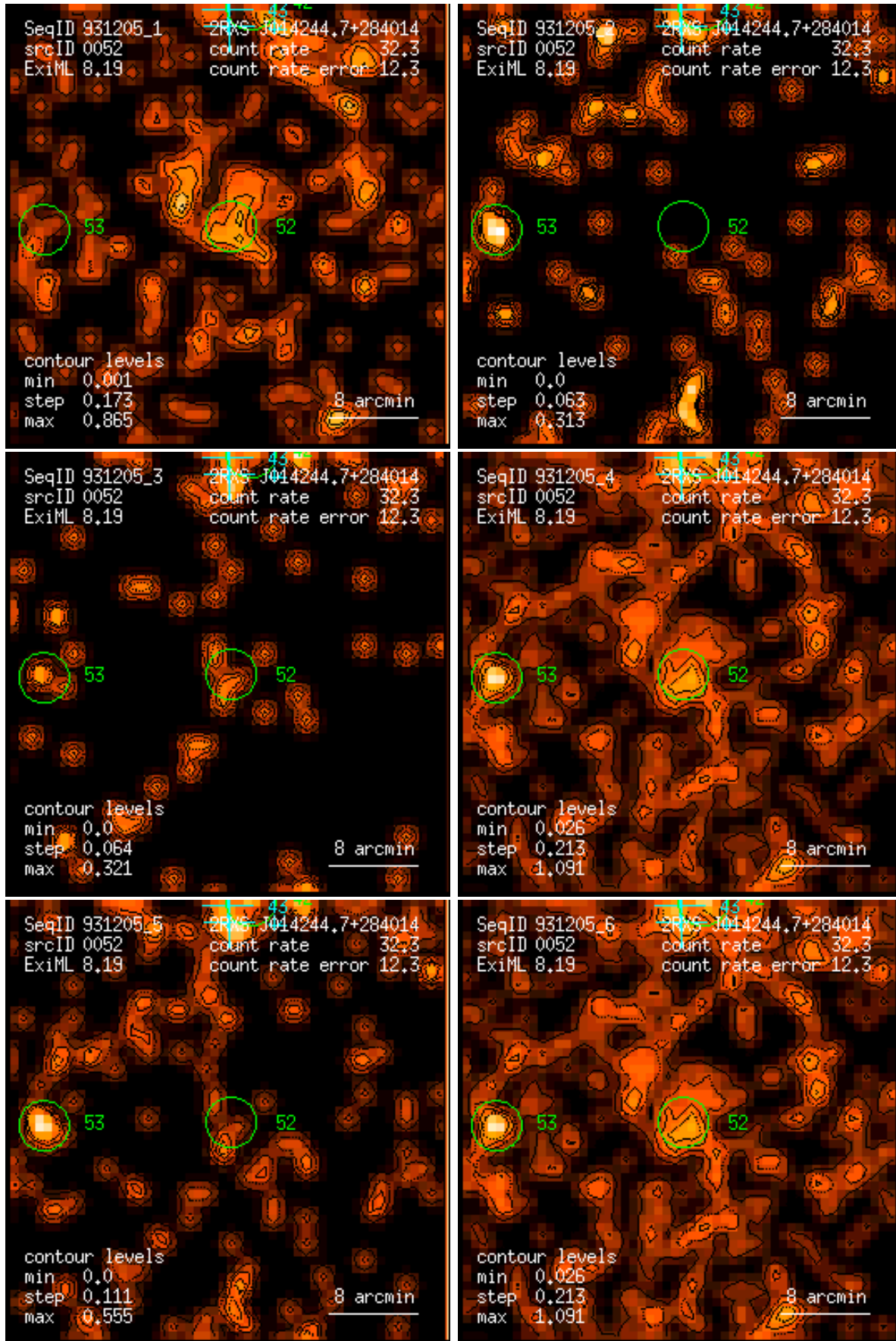
Figure 52: RASS 931205: detection 0052: band rate images, Gaussian filter: (1) PSPC channels 11 – 41, (2) 52 – 90, (3) 91 – 201, (4) 11 – 235, (5) 52 – 201, (6) 11 – 201. Broad band rates in counts/ks. Band rate contour levels in counts/ks/arcmin 2 .
