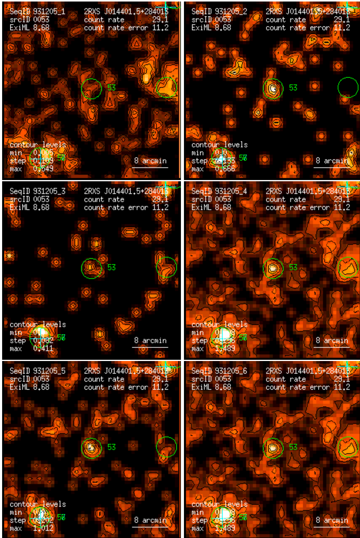
Figure 53: RASS 931205: detection 0053: band rate images, Gaussian filter: (1) PSPC channels 11 – 41, (2) 52 – 90, (3) 91 – 201, (4) 11 – 235, (5) 52 – 201, (6) 11 – 201. Broad band rates in counts/ks. Band rate contour levels in counts/ks/arcmin 2 .
