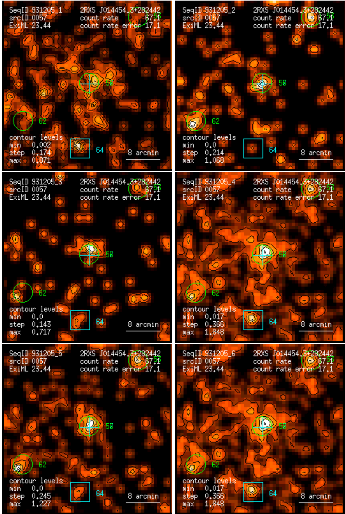
Figure 57: RASS 931205: detection 0057: band rate images, Gaussian filter: (1) PSPC channels 11 – 41, (2) 52 – 90, (3) 91 – 201, (4) 11 – 235, (5) 52 – 201, (6) 11 – 201. Broad band rates in counts/ks. Band rate contour levels in counts/ks/arcmin 2 .
