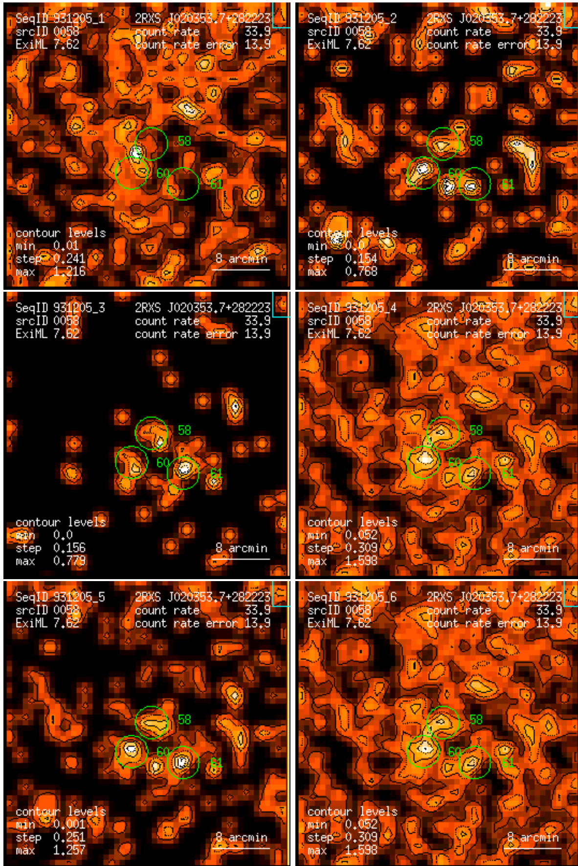
Figure 58: RASS 931205: detection 0058: band rate images, Gaussian filter: (1) PSPC channels 11 – 41, (2) 52 – 90, (3) 91 – 201, (4) 11 – 235, (5) 52 – 201, (6) 11 – 201. Broad band rates in counts/ks. Band rate contour levels in counts/ks/arcmin 2 .
