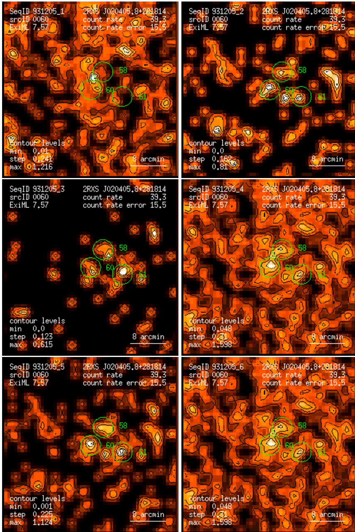
Figure 60: RASS 931205: detection 0060: band rate images, Gaussian filter: (1) PSPC channels 11 – 41, (2) 52 – 90, (3) 91 – 201, (4) 11 – 235, (5) 52 – 201, (6) 11 – 201. Broad band rates in counts/ks. Band rate contour levels in counts/ks/arcmin 2 .
