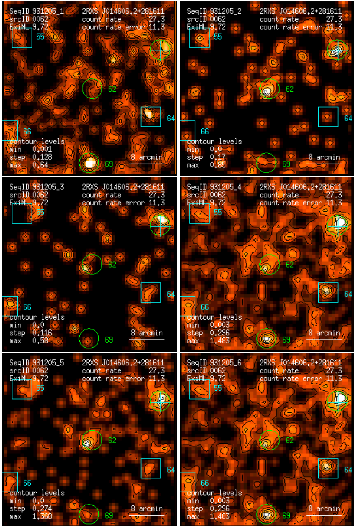
Figure 62: RASS 931205: detection 0062: band rate images, Gaussian filter: (1) PSPC channels 11 – 41, (2) 52 – 90, (3) 91 – 201, (4) 11 – 235, (5) 52 – 201, (6) 11 – 201. Broad band rates in counts/ks. Band rate contour levels in counts/ks/arcmin 2 .
