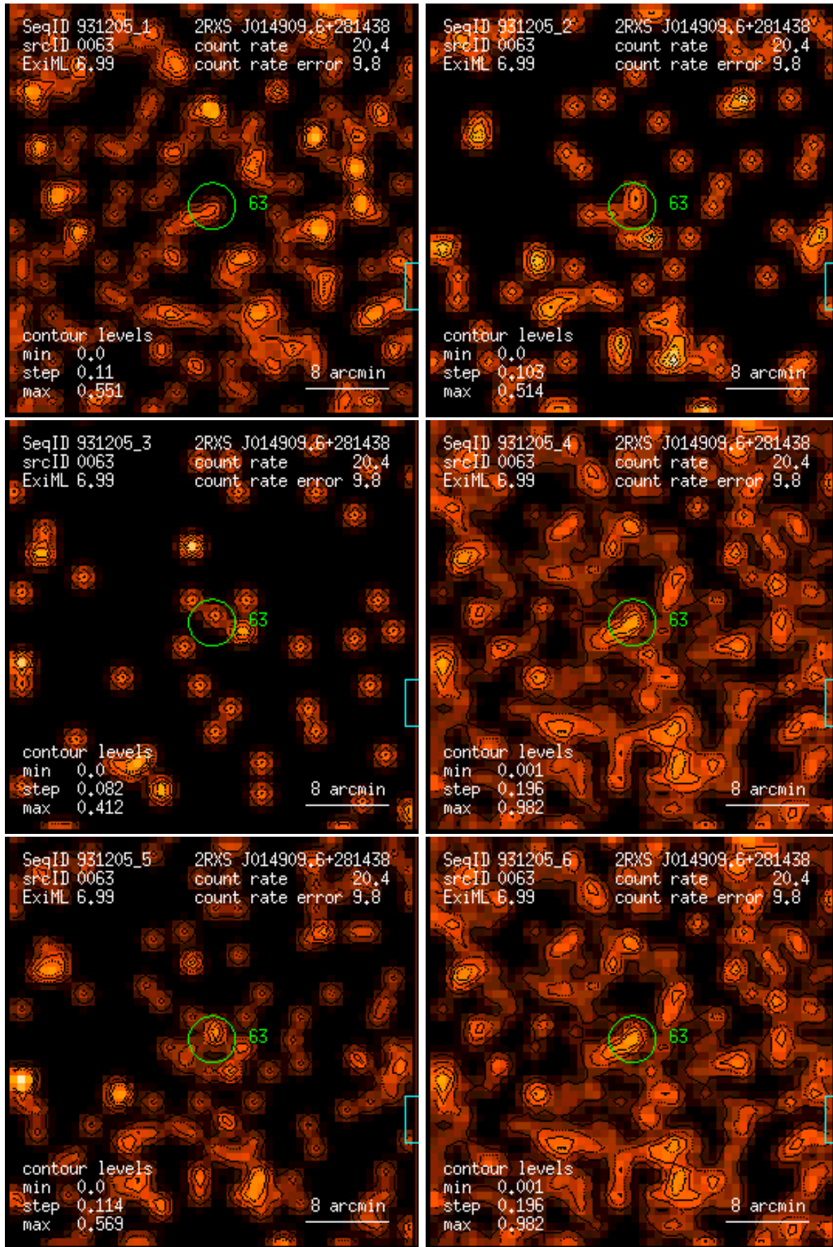
Figure 63: RASS 931205: detection 0063: band rate images, Gaussian filter: (1) PSPC channels 11 – 41, (2) 52 – 90, (3) 91 – 201, (4) 11 – 235, (5) 52 – 201, (6) 11 – 201. Broad band rates in counts/ks. Band rate contour levels in counts/ks/arcmin 2 .
