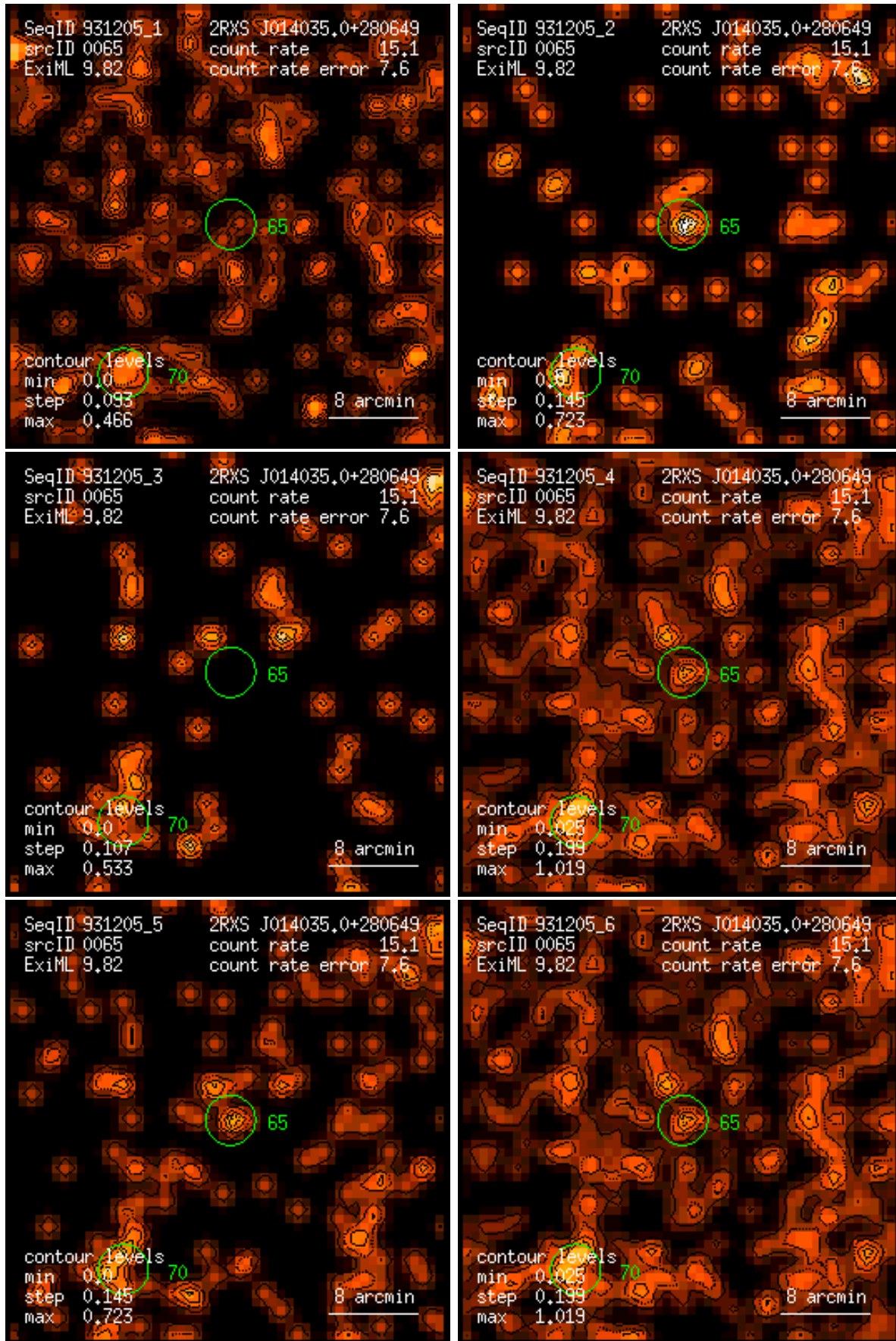
Figure 65: RASS 931205: detection 0065: band rate images, Gaussian filter: (1) PSPC channels 11 – 41, (2) 52 – 90, (3) 91 – 201, (4) 11 – 235, (5) 52 – 201, (6) 11 – 201. Broad band rates in counts/ks. Band rate contour levels in counts/ks/arcmin 2 .
