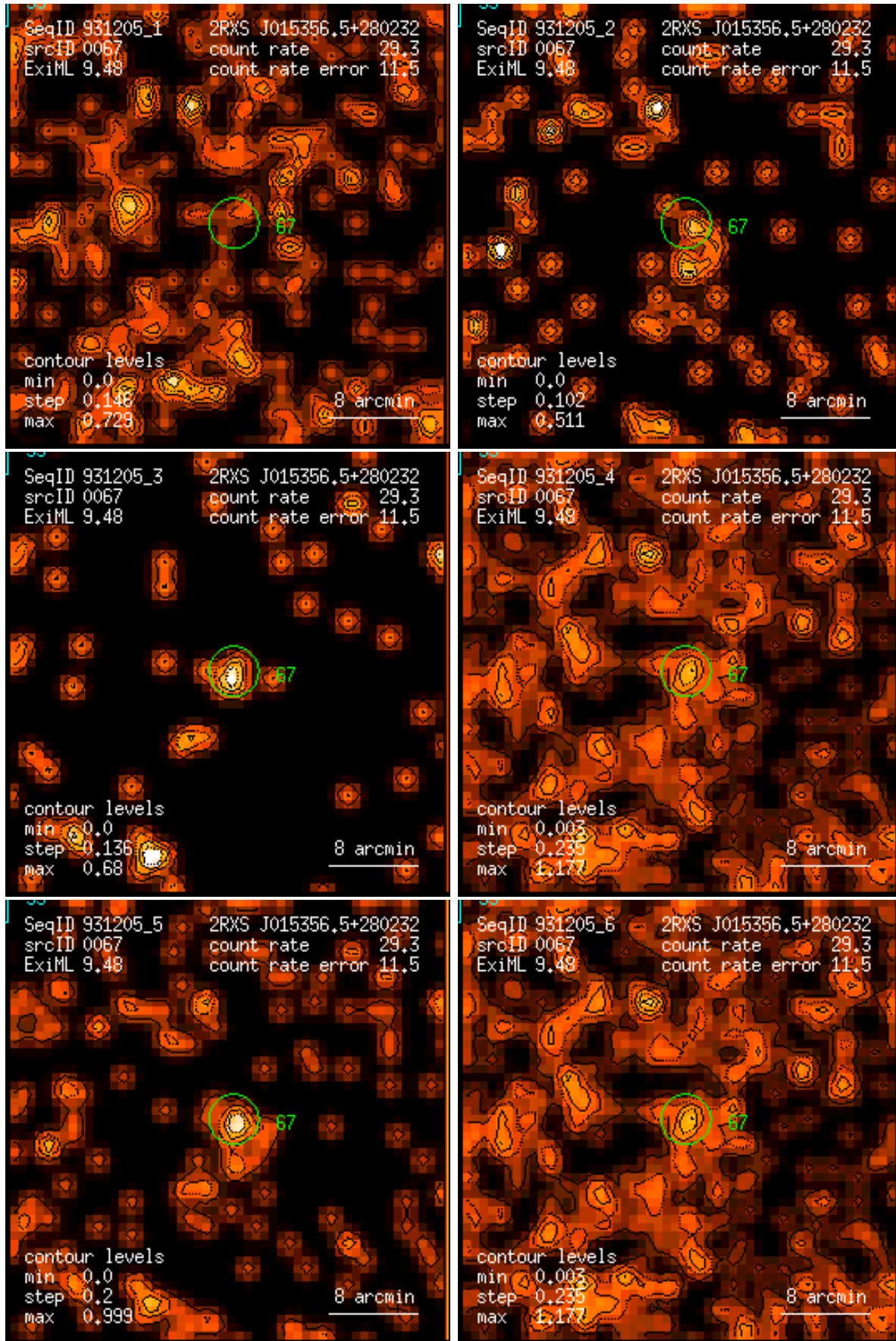
Figure 67: RASS 931205: detection 0067: band rate images, Gaussian filter: (1) PSPC channels 11 – 41, (2) 52 – 90, (3) 91 – 201, (4) 11 – 235, (5) 52 – 201, (6) 11 – 201. Broad band rates in counts/ks. Band rate contour levels in counts/ks/arcmin 2 .
