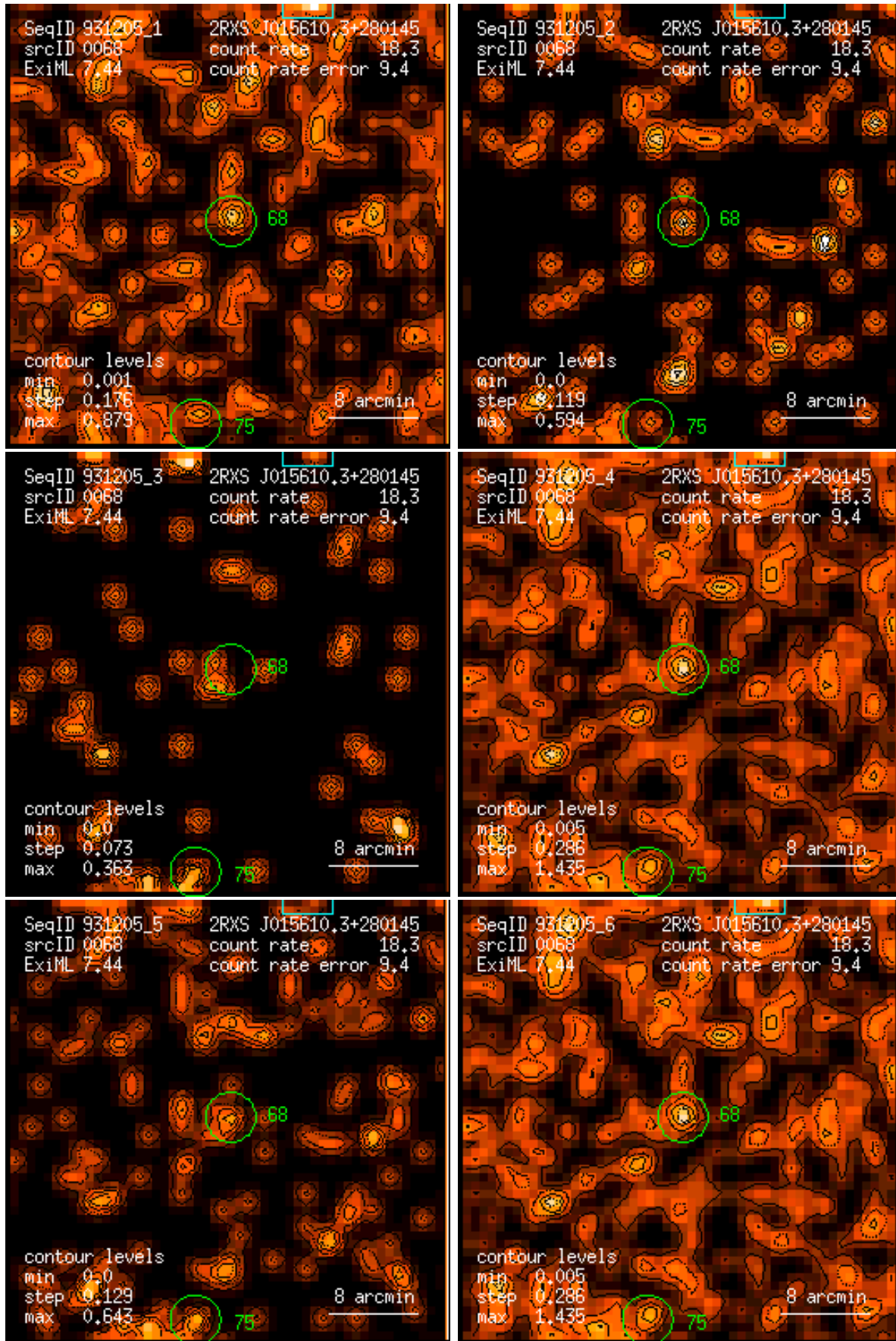
Figure 68: RASS 931205: detection 0068: band rate images, Gaussian filter: (1) PSPC channels 11 – 41, (2) 52 – 90, (3) 91 – 201, (4) 11 – 235, (5) 52 – 201, (6) 11 – 201. Broad band rates in counts/ks. Band rate contour levels in counts/ks/arcmin 2 .
