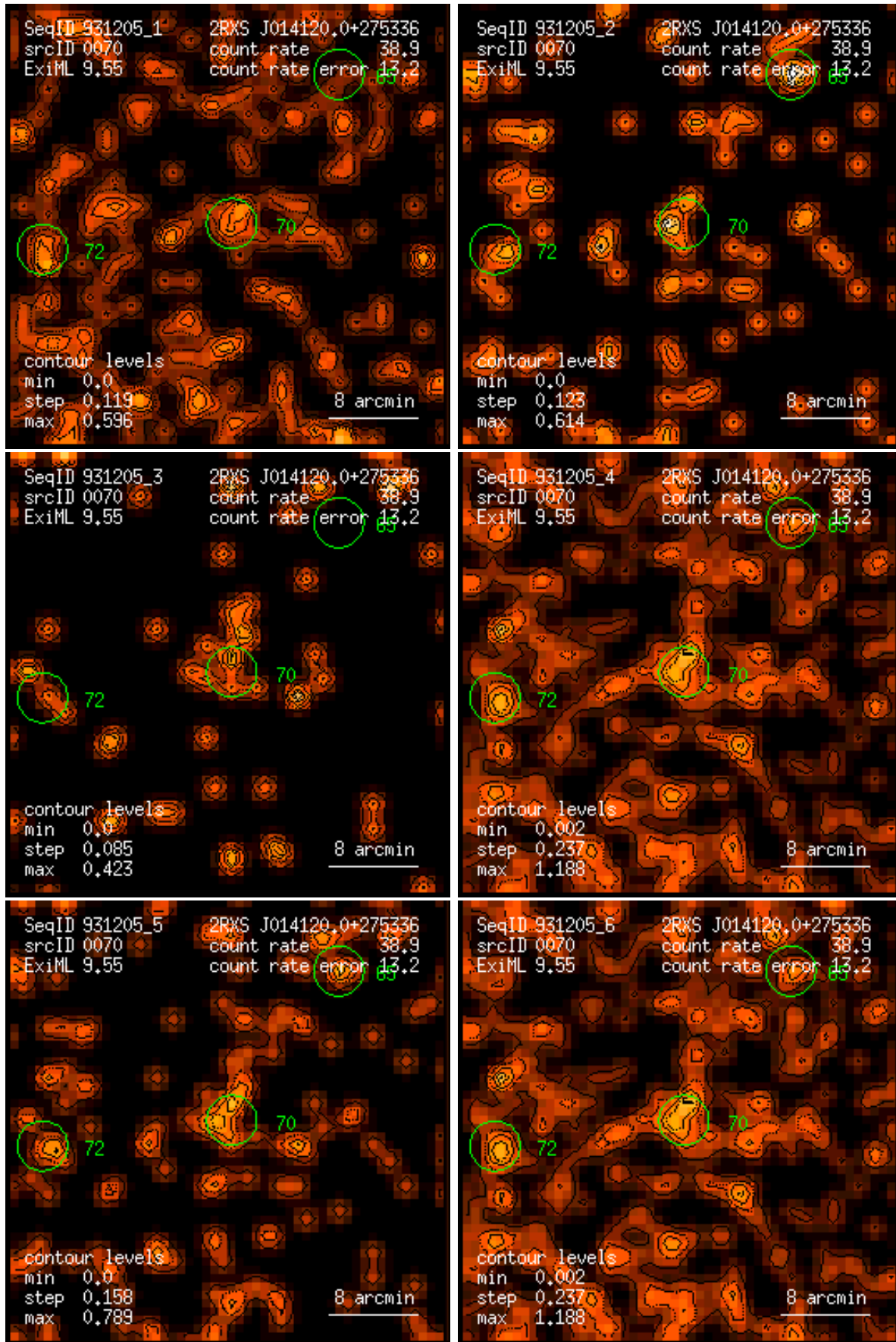
Figure 70: RASS 931205: detection 0070: band rate images, Gaussian filter: (1) PSPC channels 11 – 41, (2) 52 – 90, (3) 91 – 201, (4) 11 – 235, (5) 52 – 201, (6) 11 – 201. Broad band rates in counts/ks. Band rate contour levels in counts/ks/arcmin 2 .
