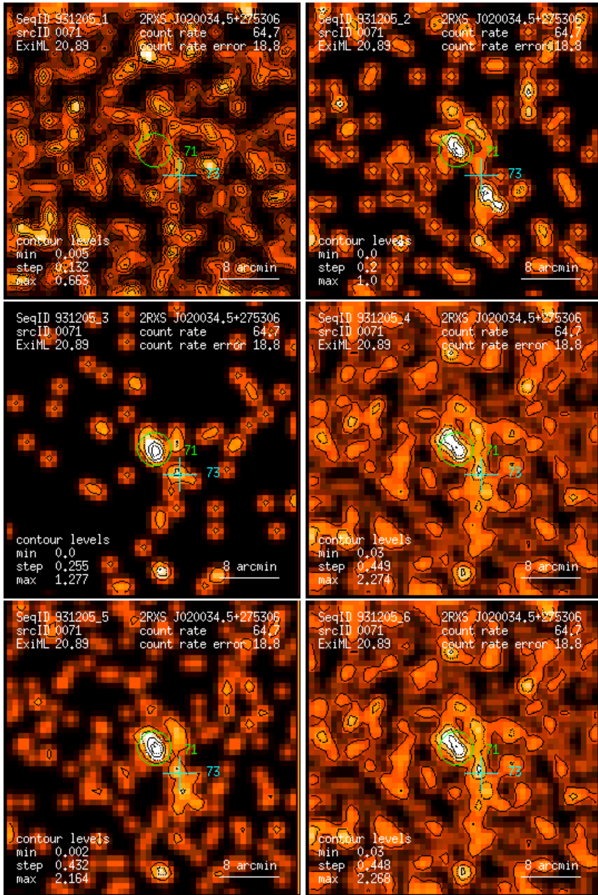
Figure 71: RASS 931205: detection 0071: band rate images, Gaussian filter: (1) PSPC channels 11 – 41, (2) 52 – 90, (3) 91 – 201, (4) 11 – 235, (5) 52 – 201, (6) 11 – 201. Broad band rates in counts/ks. Band rate contour levels in counts/ks/arcmin 2 .
