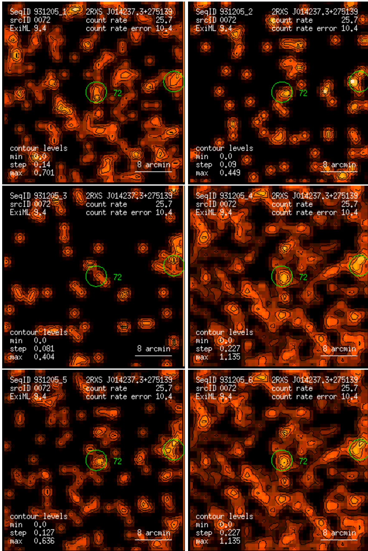
Figure 72: RASS 931205: detection 0072: band rate images, Gaussian filter: (1) PSPC channels 11 – 41, (2) 52 – 90, (3) 91 – 201, (4) 11 – 235, (5) 52 – 201, (6) 11 – 201. Broad band rates in counts/ks. Band rate contour levels in counts/ks/arcmin 2 .
