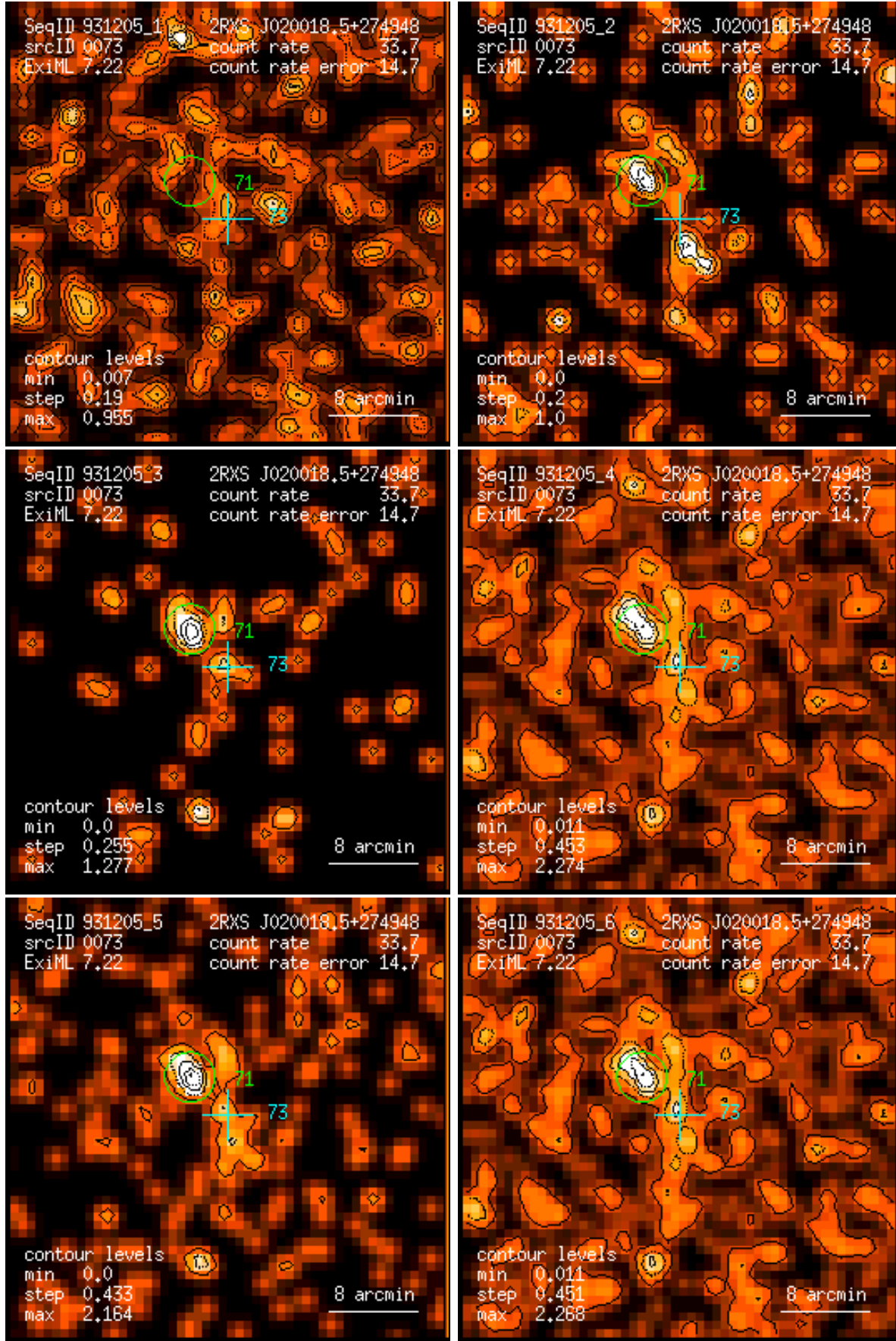
Figure 73: RASS 931205: detection 0073: band rate images, Gaussian filter: (1) PSPC channels 11 – 41, (2) 52 – 90, (3) 91 – 201, (4) 11 – 235, (5) 52 – 201, (6) 11 – 201. Broad band rates in counts/ks. Band rate contour levels in counts/ks/arcmin 2 .
