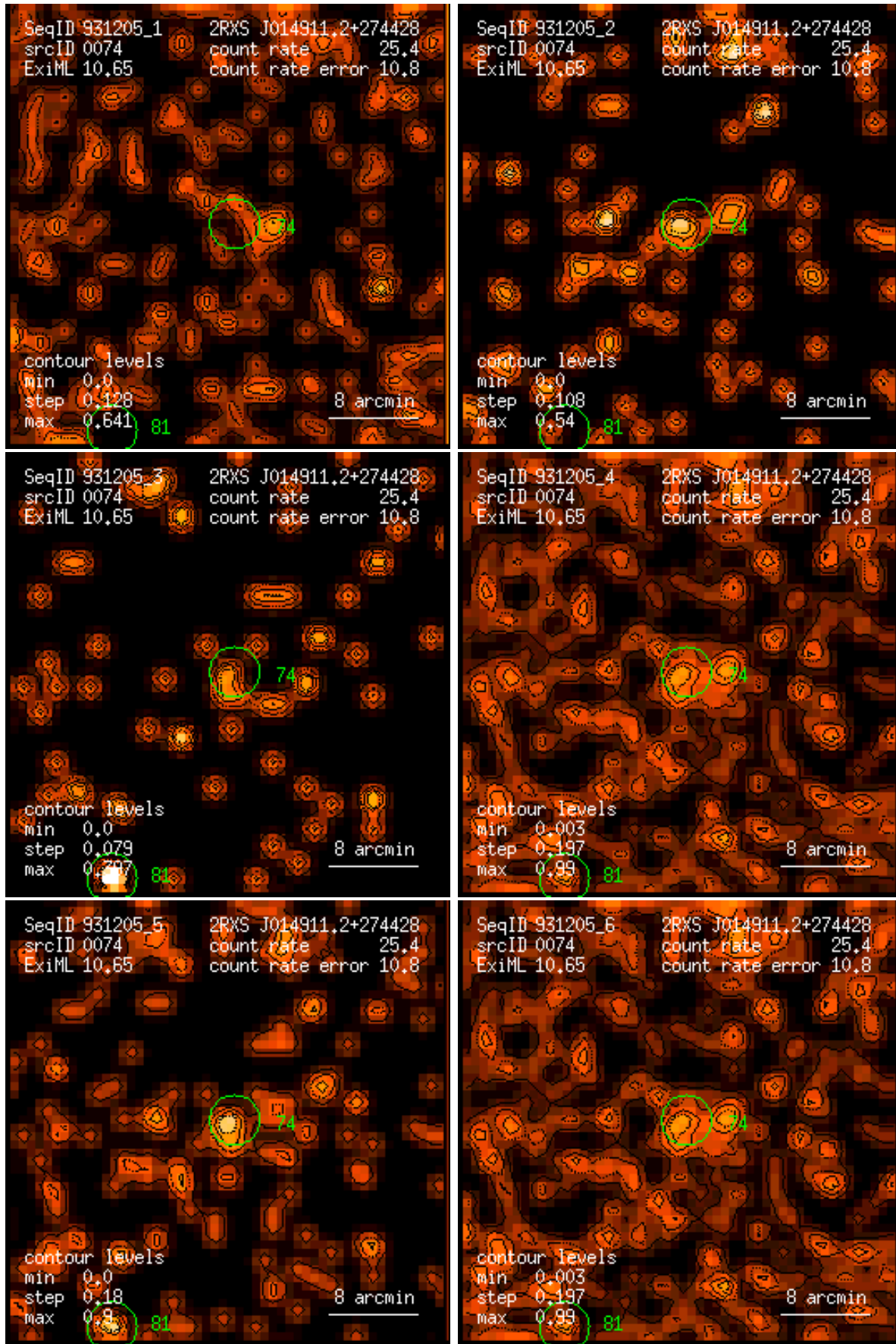
Figure 74: RASS 931205: detection 0074: band rate images, Gaussian filter: (1) PSPC channels 11 – 41, (2) 52 – 90, (3) 91 – 201, (4) 11 – 235, (5) 52 – 201, (6) 11 – 201. Broad band rates in counts/ks. Band rate contour levels in counts/ks/arcmin 2 .
