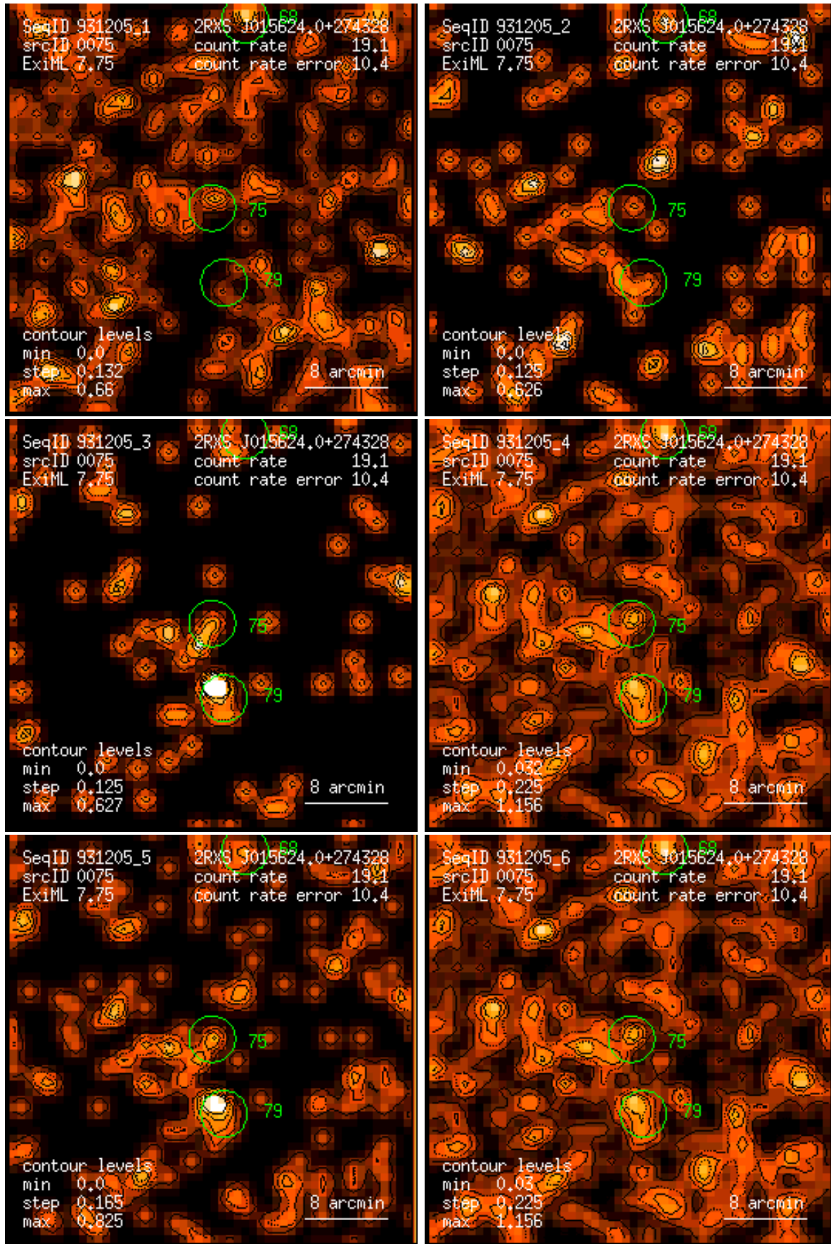
Figure 75: RASS 931205: detection 0075: band rate images, Gaussian filter: (1) PSPC channels 11 – 41, (2) 52 – 90, (3) 91 – 201, (4) 11 – 235, (5) 52 – 201, (6) 11 – 201. Broad band rates in counts/ks. Band rate contour levels in counts/ks/arcmin 2 .
