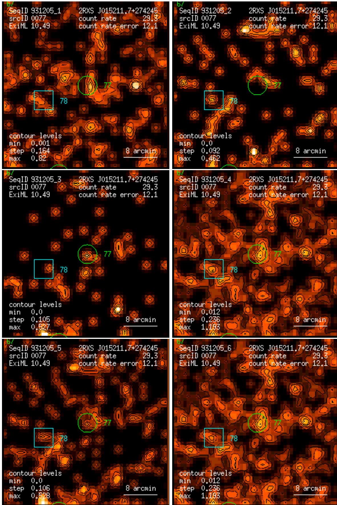
Figure 77: RASS 931205: detection 0077: band rate images, Gaussian filter: (1) PSPC channels 11 – 41, (2) 52 – 90, (3) 91 – 201, (4) 11 – 235, (5) 52 – 201, (6) 11 – 201. Broad band rates in counts/ks. Band rate contour levels in counts/ks/arcmin 2 .
