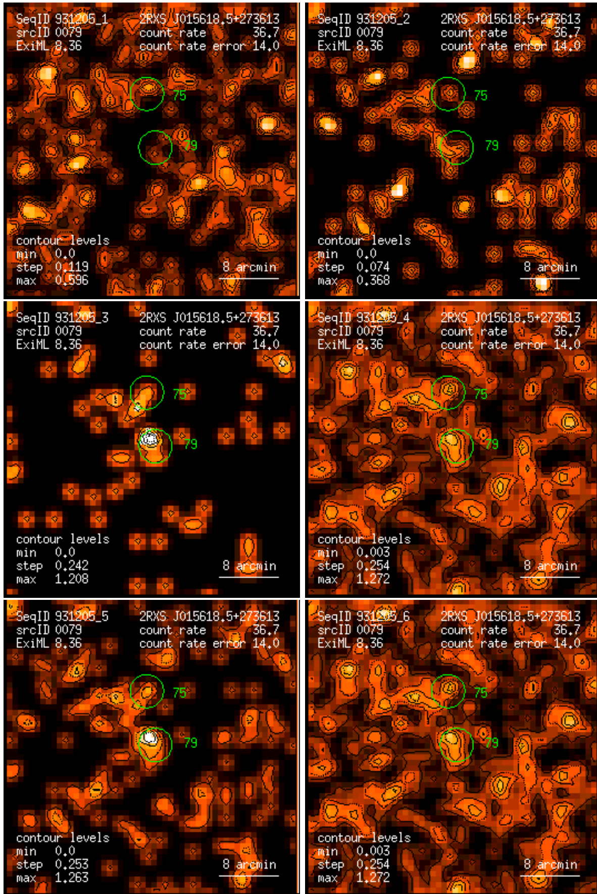
Figure 79: RASS 931205: detection 0079: band rate images, Gaussian filter: (1) PSPC channels 11 – 41, (2) 52 – 90, (3) 91 – 201, (4) 11 – 235, (5) 52 – 201, (6) 11 – 201. Broad band rates in counts/ks. Band rate contour levels in counts/ks/arcmin 2 .
