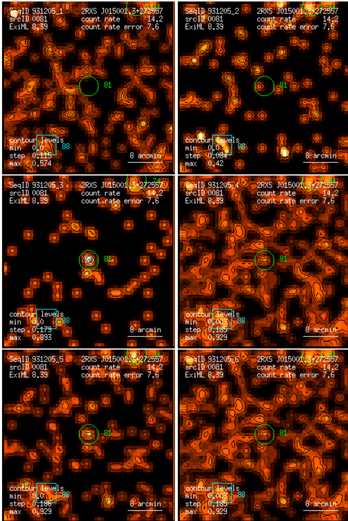
Figure 81: RASS 931205: detection 0081: band rate images, Gaussian filter: (1) PSPC channels 11 – 41, (2) 52 – 90, (3) 91 – 201, (4) 11 – 235, (5) 52 – 201, (6) 11 – 201. Broad band rates in counts/ks. Band rate contour levels in counts/ks/arcmin 2 .
