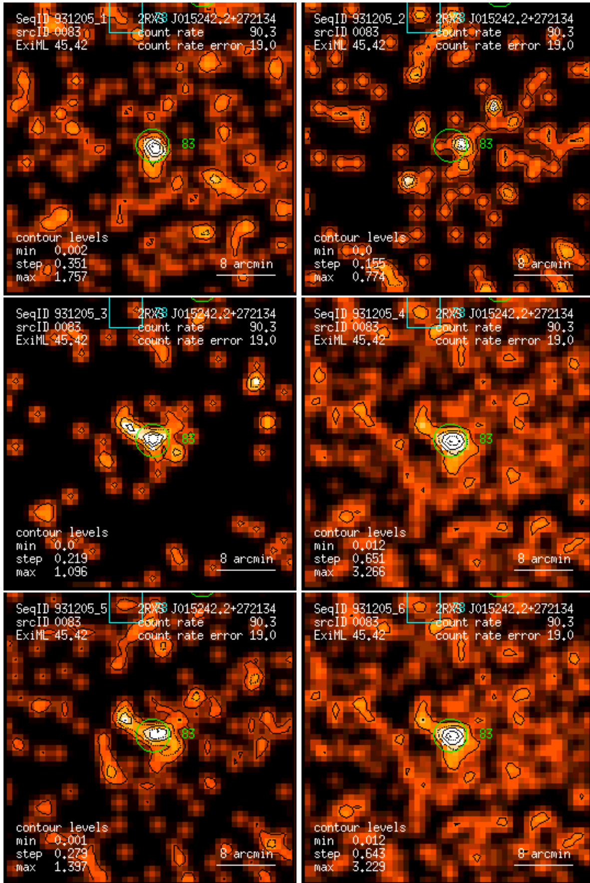
Figure 83: RASS 931205: detection 0083: band rate images, Gaussian filter: (1) PSPC channels 11 – 41, (2) 52 – 90, (3) 91 – 201, (4) 11 – 235, (5) 52 – 201, (6) 11 – 201. Broad band rates in counts/ks. Band rate contour levels in counts/ks/arcmin 2 .
