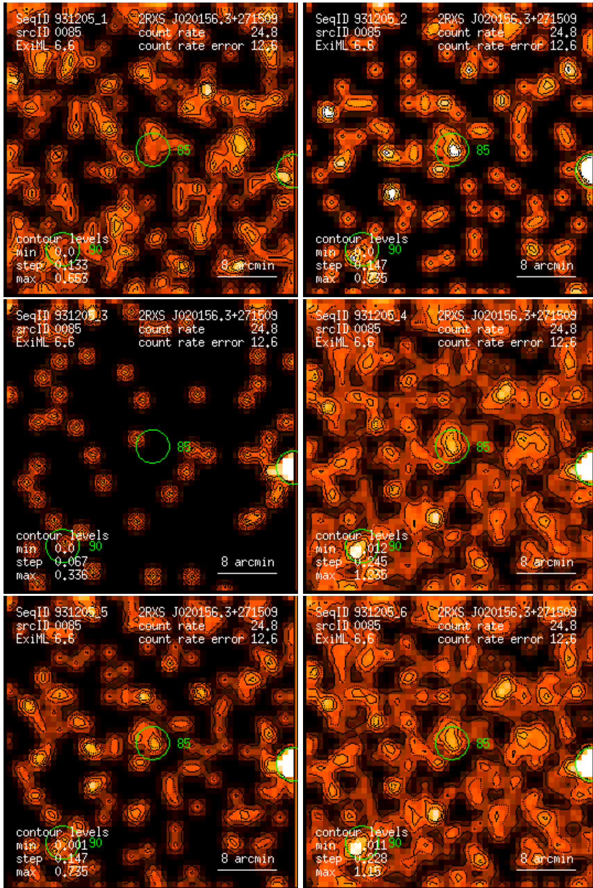
Figure 85: RASS 931205: detection 0085: band rate images, Gaussian filter: (1) PSPC channels 11 – 41, (2) 52 – 90, (3) 91 – 201, (4) 11 – 235, (5) 52 – 201, (6) 11 – 201. Broad band rates in counts/ks. Band rate contour levels in counts/ks/arcmin 2 .
