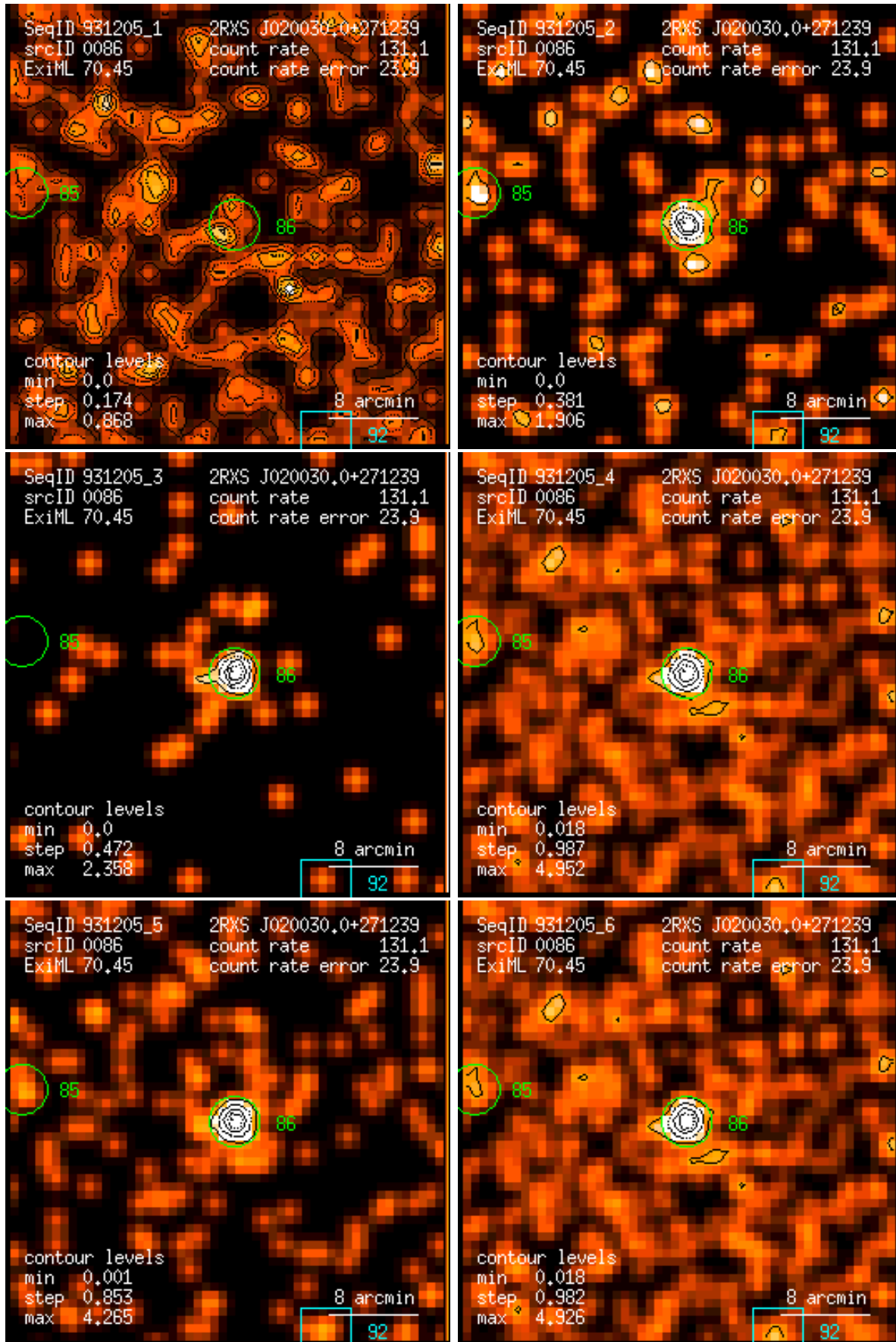
Figure 86: RASS 931205: detection 0086: band rate images, Gaussian filter: (1) PSPC channels 11 – 41, (2) 52 – 90, (3) 91 – 201, (4) 11 – 235, (5) 52 – 201, (6) 11 – 201. Broad band rates in counts/ks. Band rate contour levels in counts/ks/arcmin 2 .
