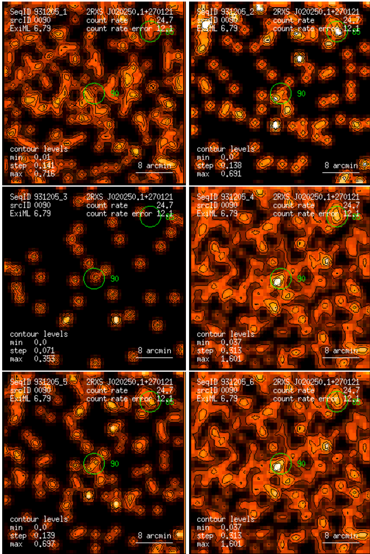
Figure 90: RASS 931205: detection 0090: band rate images, Gaussian filter: (1) PSPC channels 11 – 41, (2) 52 – 90, (3) 91 – 201, (4) 11 – 235, (5) 52 – 201, (6) 11 – 201. Broad band rates in counts/ks. Band rate contour levels in counts/ks/arcmin 2 .
