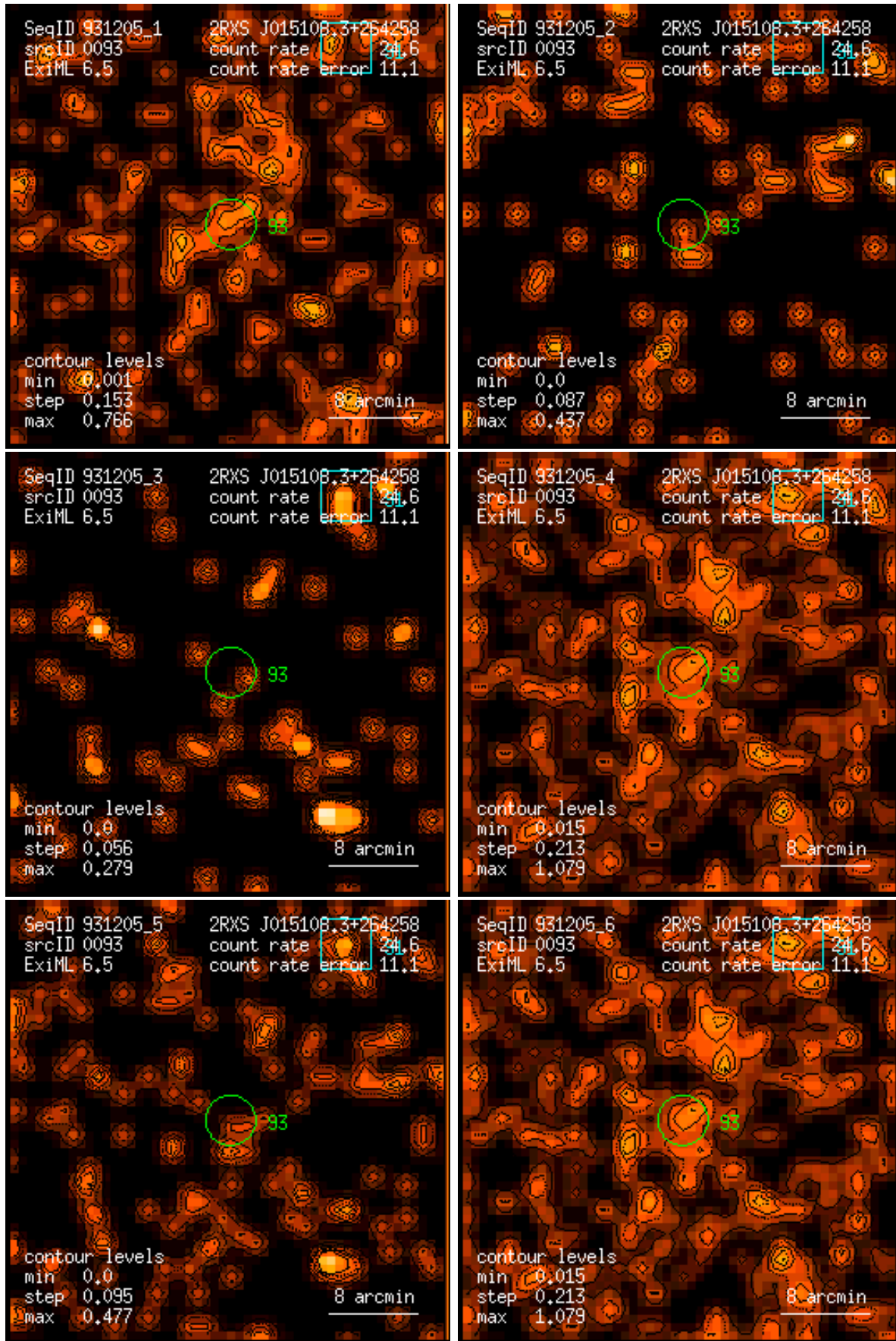
Figure 93: RASS 931205: detection 0093: band rate images, Gaussian filter: (1) PSPC channels 11 – 41, (2) 52 – 90, (3) 91 – 201, (4) 11 – 235, (5) 52 – 201, (6) 11 – 201. Broad band rates in counts/ks. Band rate contour levels in counts/ks/arcmin 2 .
