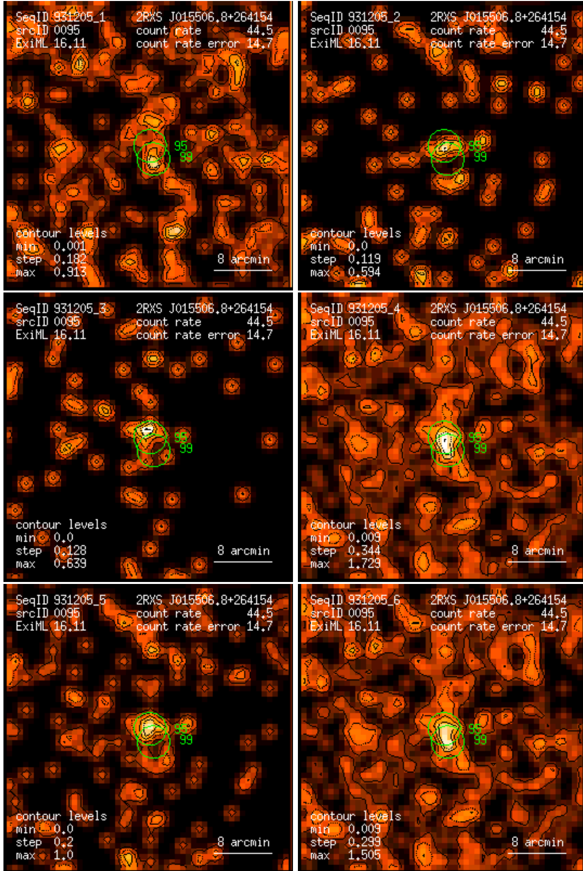
Figure 95: RASS 931205: detection 0095: band rate images, Gaussian filter: (1) PSPC channels 11 – 41, (2) 52 – 90, (3) 91 – 201, (4) 11 – 235, (5) 52 – 201, (6) 11 – 201. Broad band rates in counts/ks. Band rate contour levels in counts/ks/arcmin 2 .
