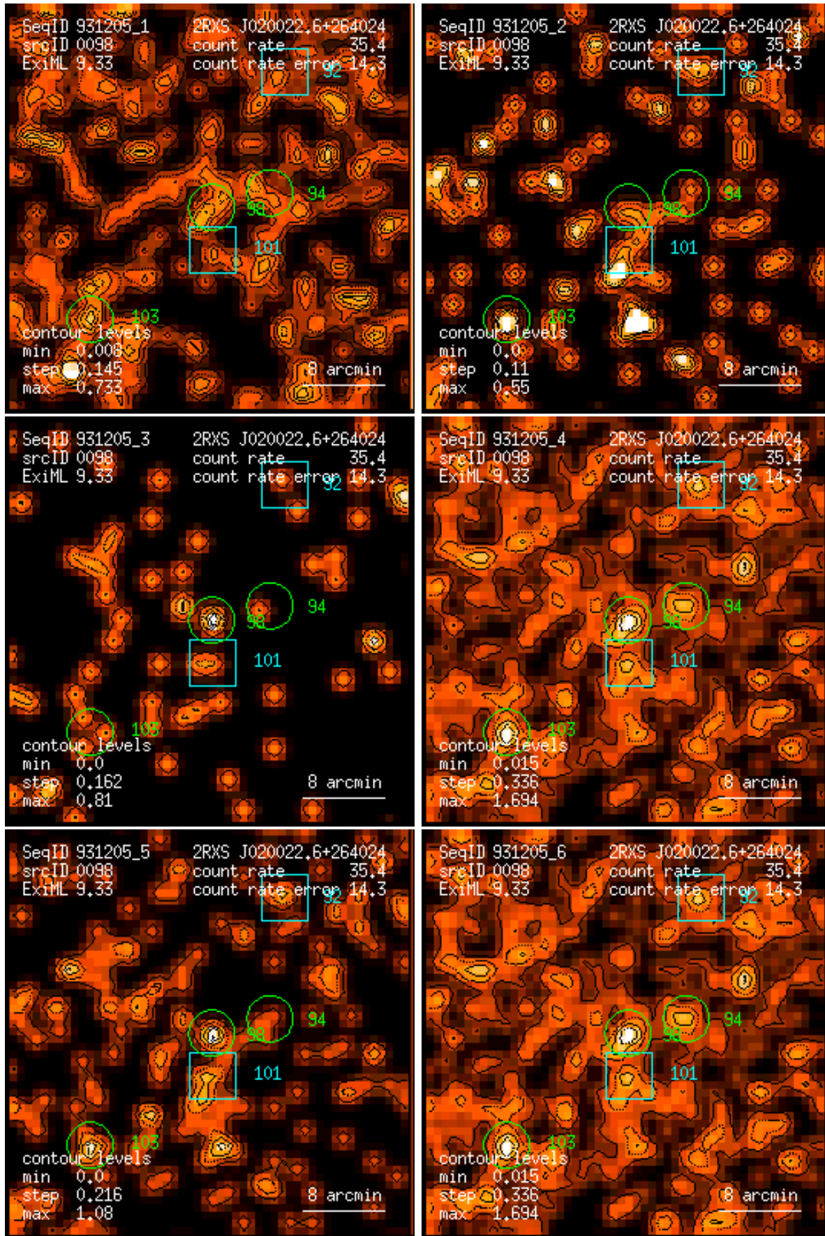
Figure 98: RASS 931205: detection 0098: band rate images, Gaussian filter: (1) PSPC channels 11 – 41, (2) 52 – 90, (3) 91 – 201, (4) 11 – 235, (5) 52 – 201, (6) 11 – 201. Broad band rates in counts/ks. Band rate contour levels in counts/ks/arcmin 2 .
