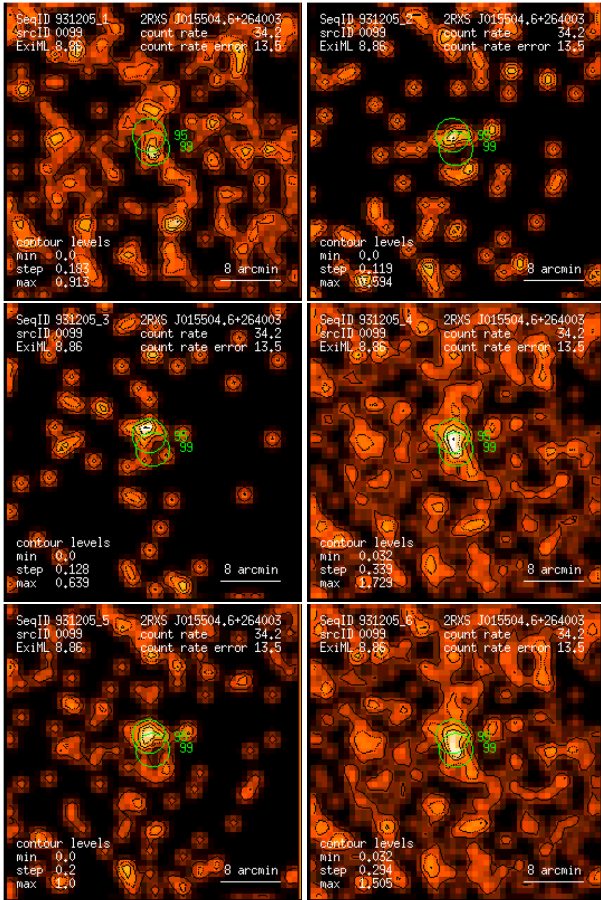
Figure 99: RASS 931205: detection 0099: band rate images, Gaussian filter: (1) PSPC channels 11 – 41, (2) 52 – 90, (3) 91 – 201, (4) 11 – 235, (5) 52 – 201, (6) 11 – 201. Broad band rates in counts/ks. Band rate contour levels in counts/ks/arcmin 2 .
