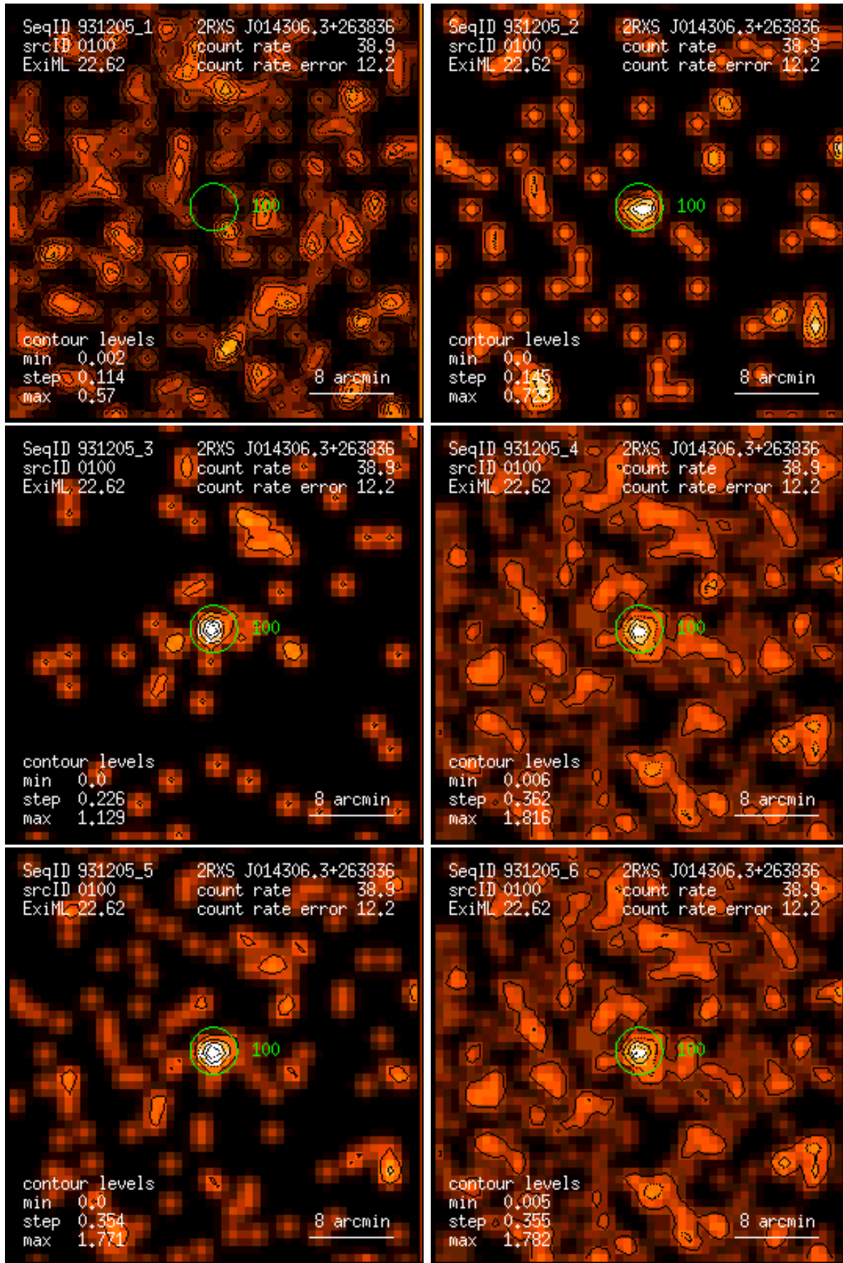
Figure 100: RASS 931205: detection 0100: band rate images, Gaussian filter: (1) PSPC channels 11 – 41, (2) 52 – 90, (3) 91 – 201, (4) 11 – 235, (5) 52 – 201, (6) 11 – 201. Broad band rates in counts/ks. Band rate contour levels in counts/ks/arcmin 2 .
