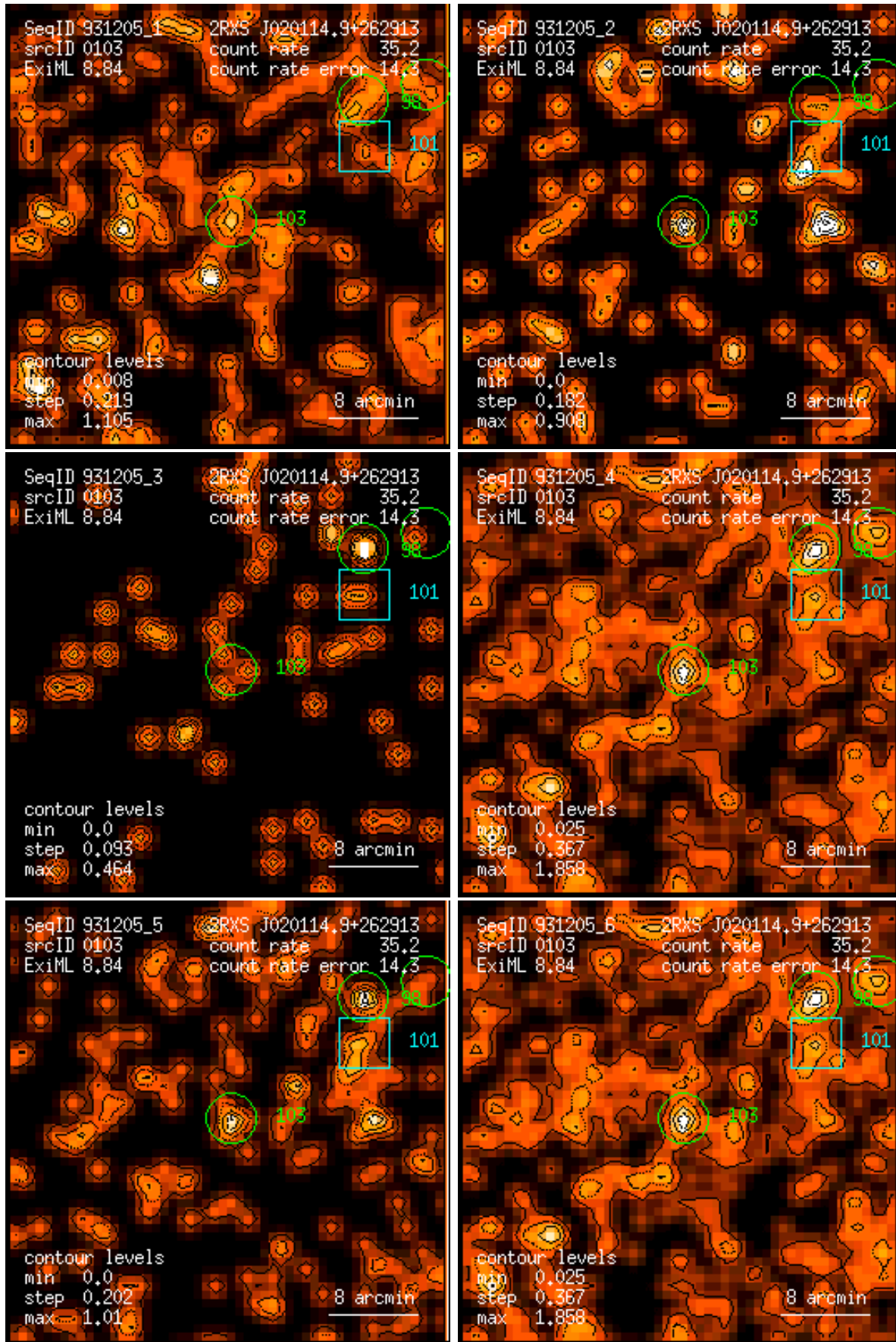
Figure 103: RASS 931205: detection 0103: band rate images, Gaussian filter: (1) PSPC channels 11 – 41, (2) 52 – 90, (3) 91 – 201, (4) 11 – 235, (5) 52 – 201, (6) 11 – 201. Broad band rates in counts/ks. Band rate contour levels in counts/ks/arcmin 2 .
