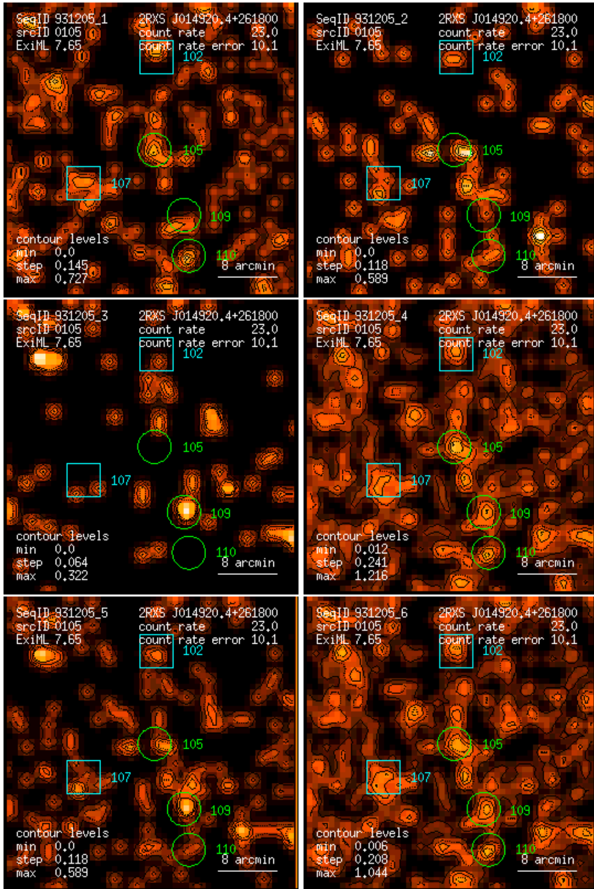
Figure 105: RASS 931205: detection 0105: band rate images, Gaussian filter: (1) PSPC channels 11 – 41, (2) 52 – 90, (3) 91 – 201, (4) 11 – 235, (5) 52 – 201, (6) 11 – 201. Broad band rates in counts/ks. Band rate contour levels in counts/ks/arcmin 2 .
