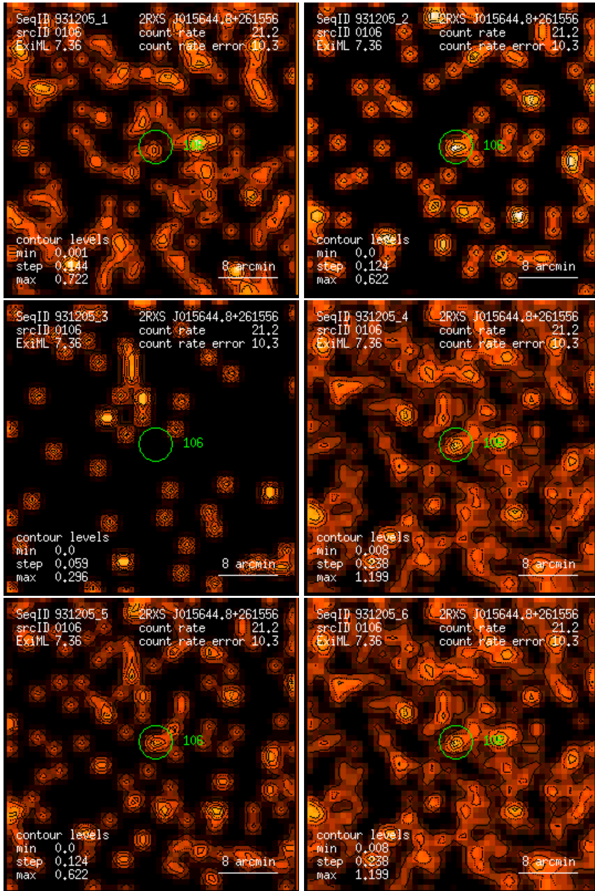
Figure 106: RASS 931205: detection 0106: band rate images, Gaussian filter: (1) PSPC channels 11 – 41, (2) 52 – 90, (3) 91 – 201, (4) 11 – 235, (5) 52 – 201, (6) 11 – 201. Broad band rates in counts/ks. Band rate contour levels in counts/ks/arcmin 2 .
