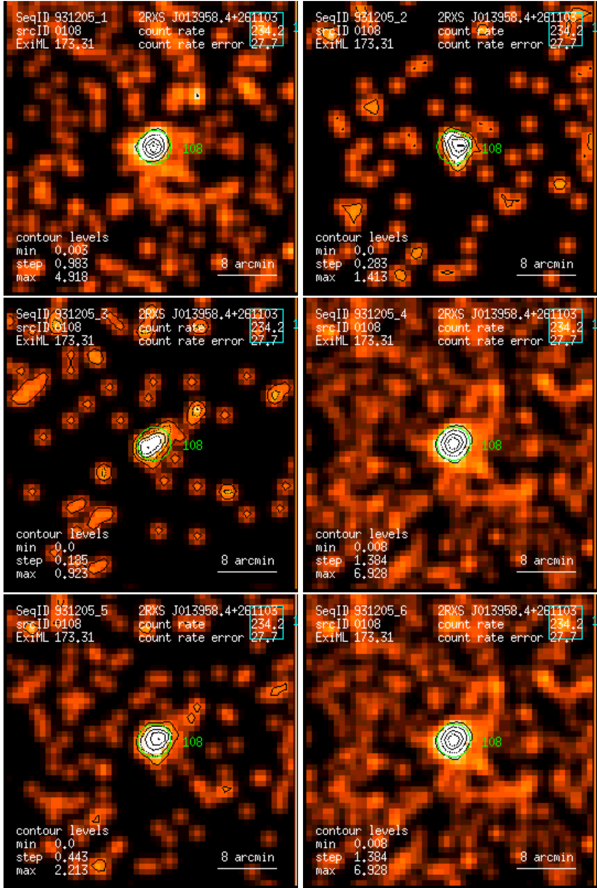
Figure 108: RASS 931205: detection 0108: band rate images, Gaussian filter: (1) PSPC channels 11 – 41, (2) 52 – 90, (3) 91 – 201, (4) 11 – 235, (5) 52 – 201, (6) 11 – 201. Broad band rates in counts/ks. Band rate contour levels in counts/ks/arcmin 2 .
