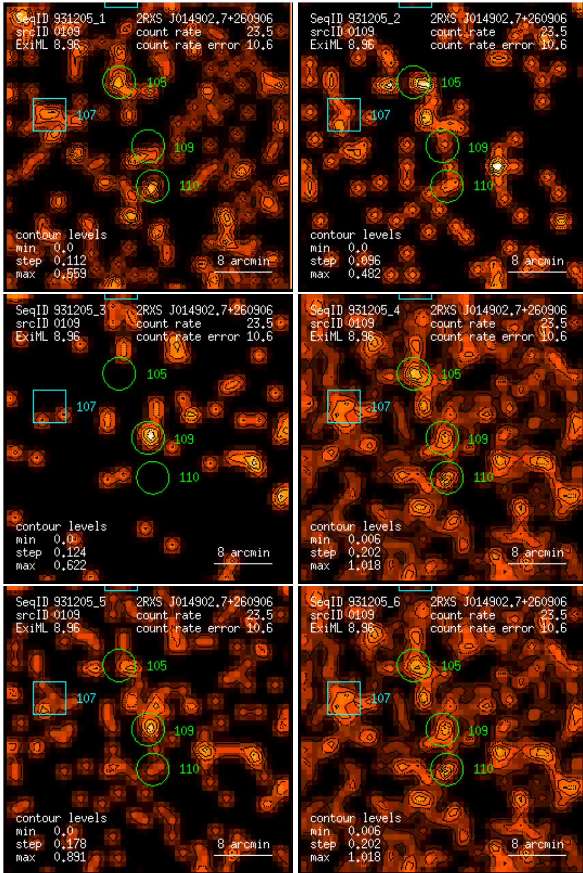
Figure 109: RASS 931205: detection 0109: band rate images, Gaussian filter: (1) PSPC channels 11 – 41, (2) 52 – 90, (3) 91 – 201, (4) 11 – 235, (5) 52 – 201, (6) 11 – 201. Broad band rates in counts/ks. Band rate contour levels in counts/ks/arcmin 2 .
