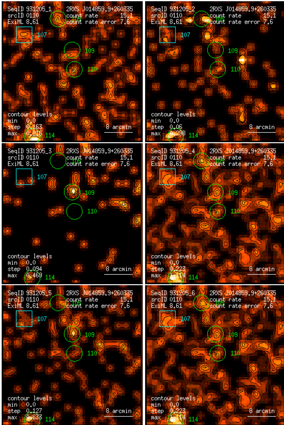
Figure 110: RASS 931205: detection 0110: band rate images, Gaussian filter: (1) PSPC channels 11 – 41, (2) 52 – 90, (3) 91 – 201, (4) 11 – 235, (5) 52 – 201, (6) 11 – 201. Broad band rates in counts/ks. Band rate contour levels in counts/ks/arcmin 2 .
