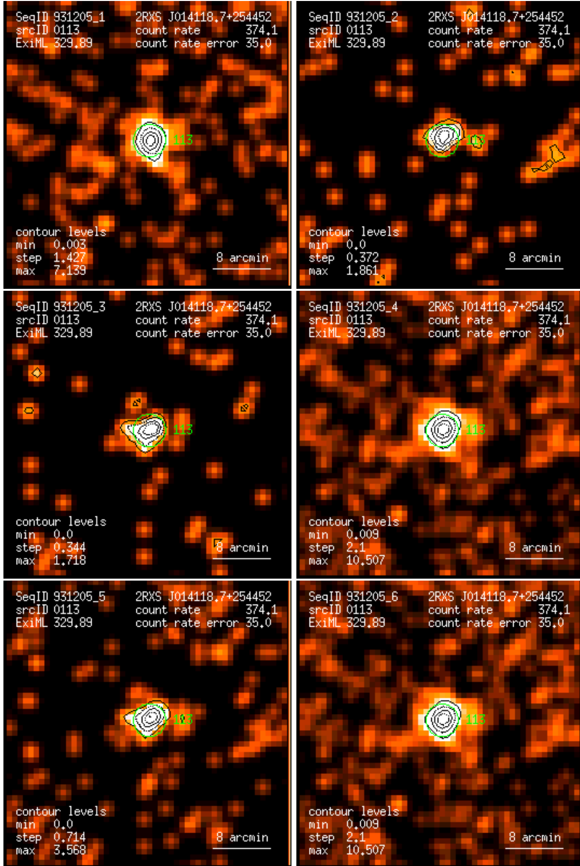
Figure 113: RASS 931205: detection 0113: band rate images, Gaussian filter: (1) PSPC channels 11 – 41, (2) 52 – 90, (3) 91 – 201, (4) 11 – 235, (5) 52 – 201, (6) 11 – 201. Broad band rates in counts/ks. Band rate contour levels in counts/ks/arcmin 2 .
