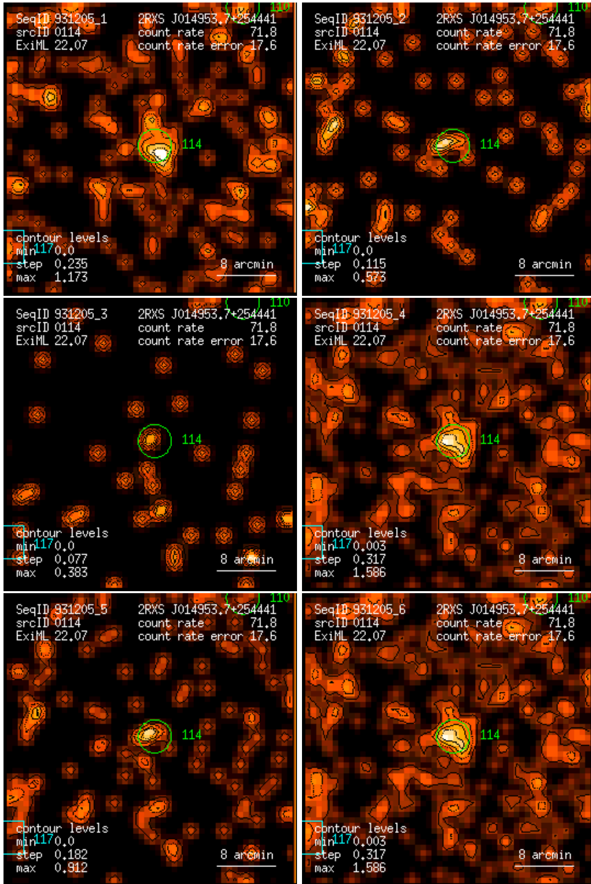
Figure 114: RASS 931205: detection 0114: band rate images, Gaussian filter: (1) PSPC channels 11 – 41, (2) 52 – 90, (3) 91 – 201, (4) 11 – 235, (5) 52 – 201, (6) 11 – 201. Broad band rates in counts/ks. Band rate contour levels in counts/ks/arcmin 2 .
