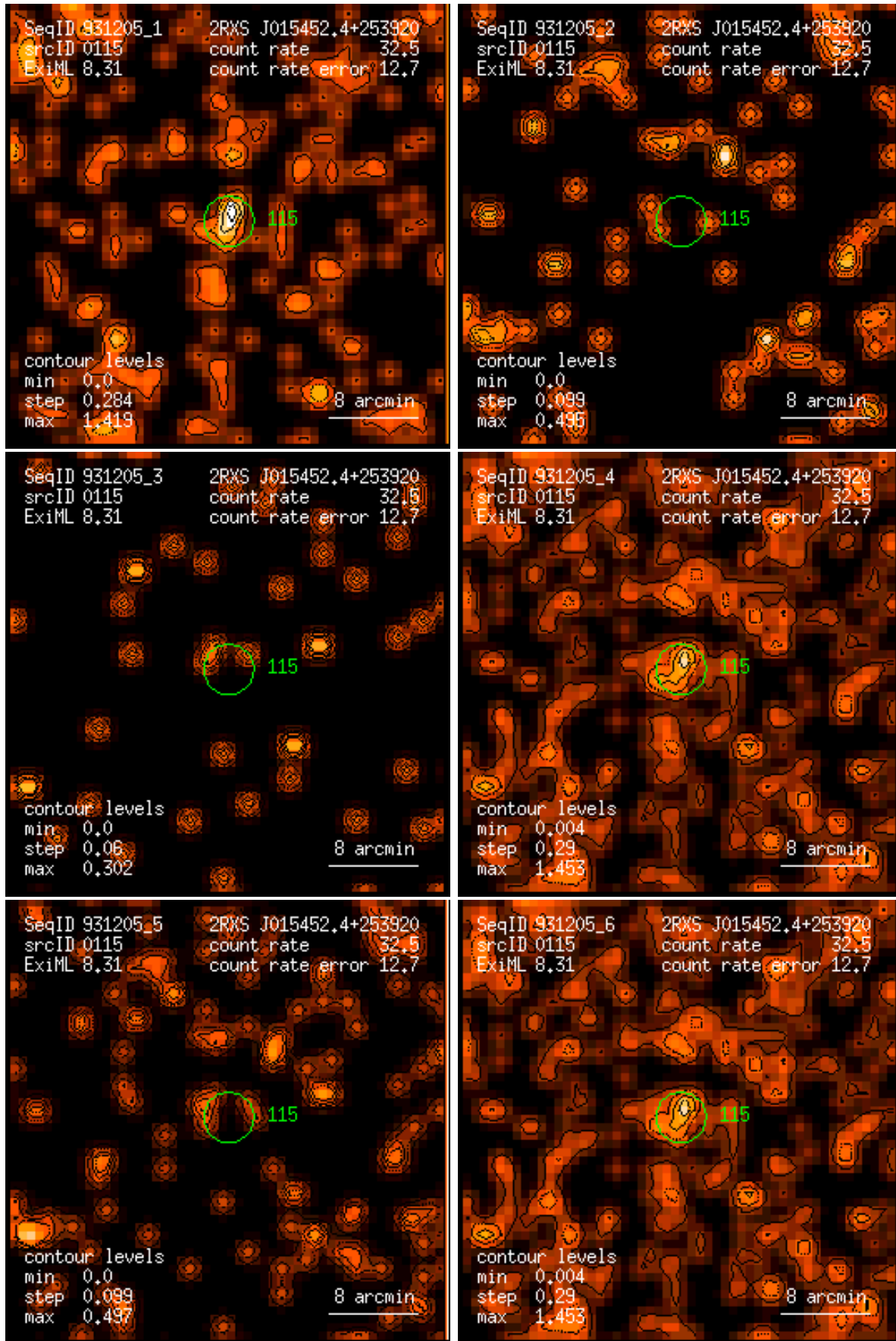
Figure 115: RASS 931205: detection 0115: band rate images, Gaussian filter: (1) PSPC channels 11 – 41, (2) 52 – 90, (3) 91 – 201, (4) 11 – 235, (5) 52 – 201, (6) 11 – 201. Broad band rates in counts/ks. Band rate contour levels in counts/ks/arcmin 2 .
