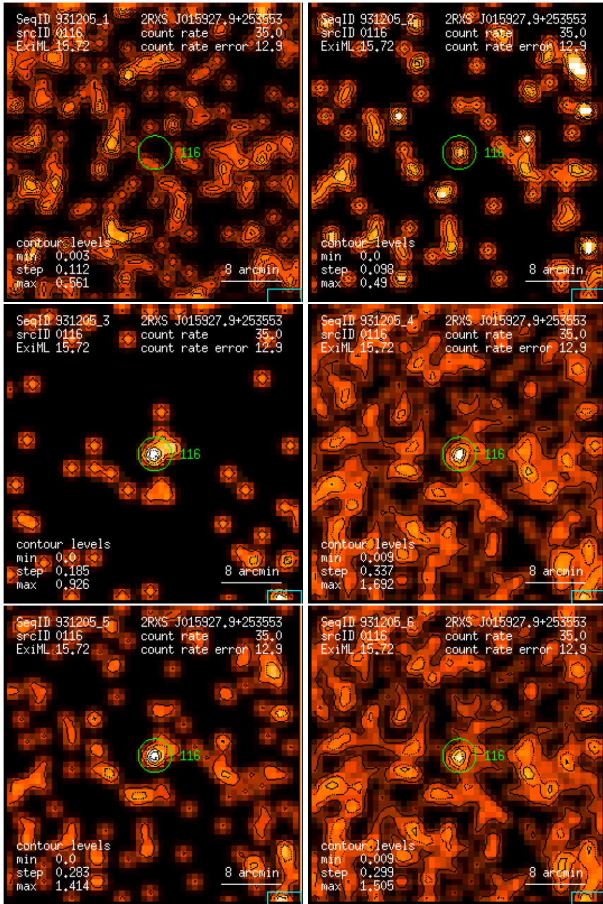
Figure 116: RASS 931205: detection 0116: band rate images, Gaussian filter: (1) PSPC channels 11 – 41, (2) 52 – 90, (3) 91 – 201, (4) 11 – 235, (5) 52 – 201, (6) 11 – 201. Broad band rates in counts/ks. Band rate contour levels in counts/ks/arcmin 2 .
