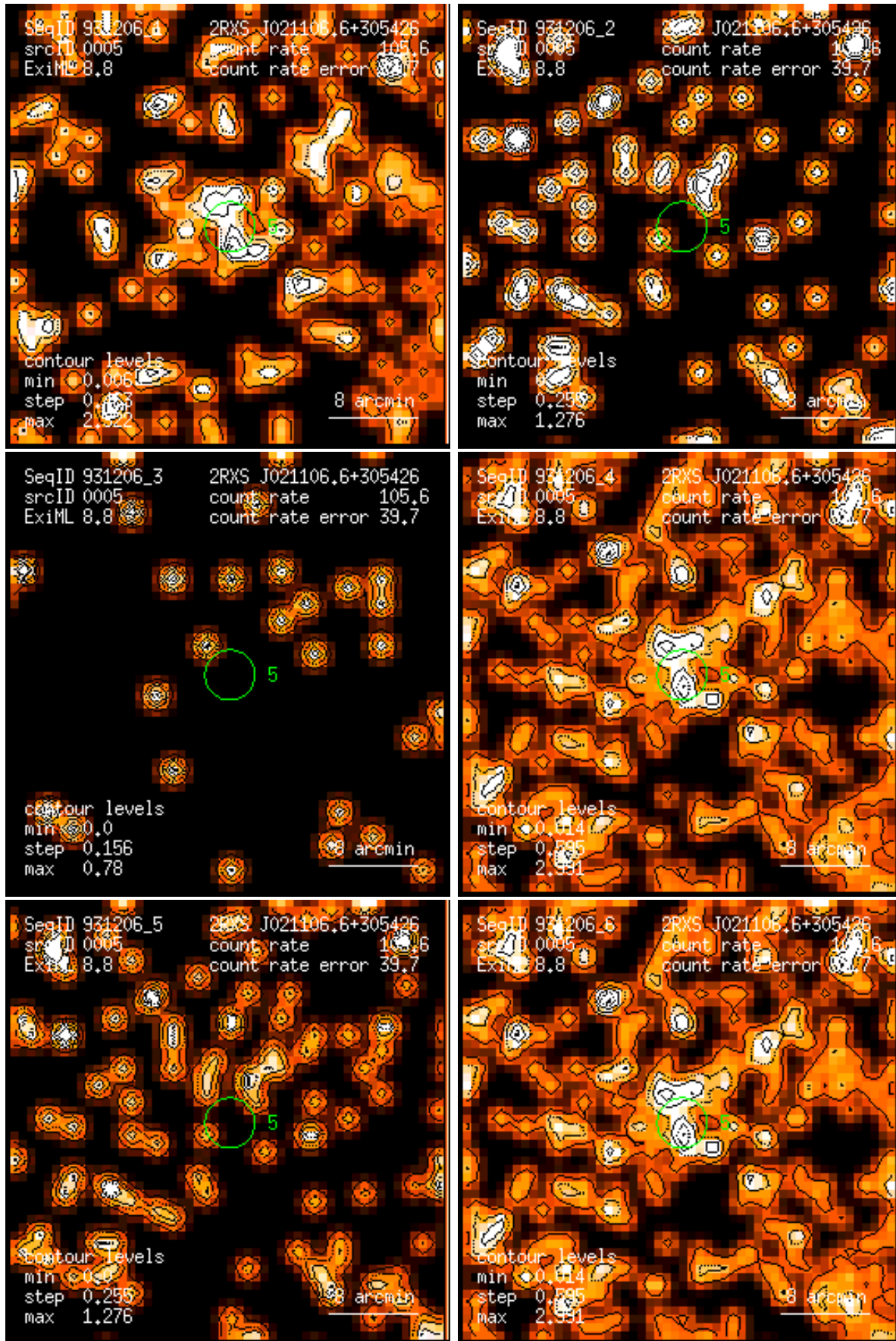
Figure 5: RASS 931206: detection 0005: band rate images, Gaussian filter: (1) PSPC channels 11 – 41, (2) 52 – 90, (3) 91 – 201, (4) 11 – 235, (5) 52 – 201, (6) 11 – 201. Broad band rates in counts/ks. Band rate contour levels in counts/ks/arcmin 2 .
